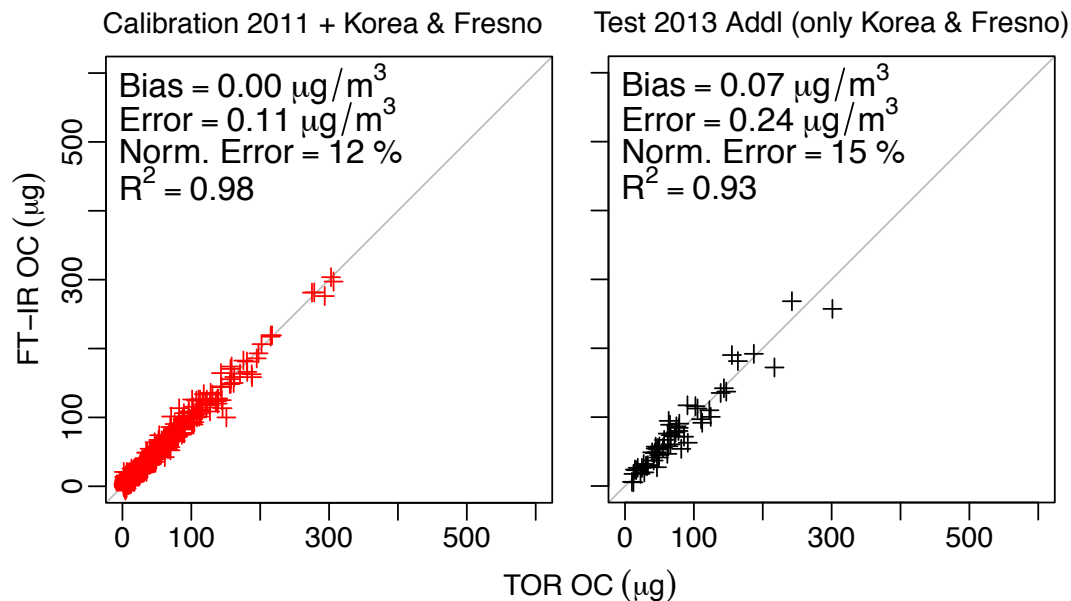
Fig. 1. Scatterplot and performance metrics between FT-IR OC and TOR OC of the Korea and Fresno sites (Site ID 10 and 11 respectively).
