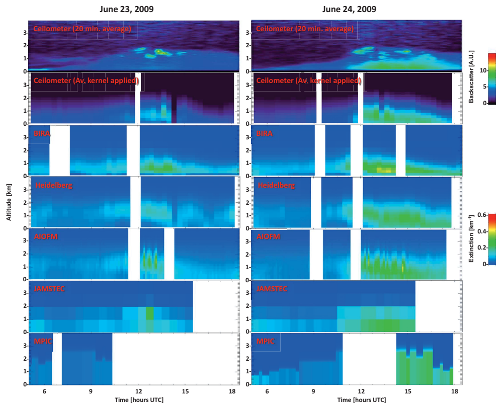
Figure 4. Comparison of MAX-DOAS extinction profiles with backscatter profiles from the ceilometer for 23 June (left) 24 June (right). The top panel shows the backscatter signal in original vertical resolution, the second panel the backscatter signal with the averaging kernels of Heidelberg applied, below the extinction profiles retrieved from BIRA, Heidelberg, JAMSTEC and MPIC. For MPIC box-profiles with the retrieved layer height and AOT are plotted.
