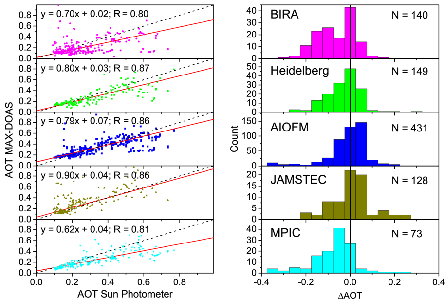
Figure 11. Left panels: correlation between AOT from the different workgroups and from the sun photometer. The red line shows the linear fit and the dashed line the 1 : 1 line. Right panels: histograms of the difference in AOT (MAX-DOAS – sun photometer).
