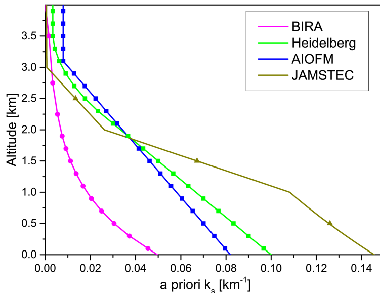
Figure 1. A priori profiles for the BIRA, Heidelberg, AIOFM and JAMSTEC retrievals. The symbols indicate the centre of each retrieval layer. The BIRA, Heidelberg and AIOFM algorithm use a 200 m vertical grid with constant extinction in each layer, and JAMSTEC a 1 km grid with exponentially decreasing extinction in each layer.
