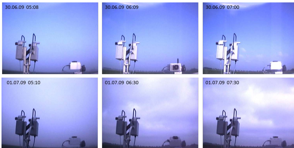
Figure 8. Webcam images from the mornings of 30 June and 1 July 2009, when foggy conditions prevailed. The webcam pointed to the viewing direction of the MAX-DOAS Instruments (north-east). The devices in the foreground are the telescopes of the Heidelberg group.
