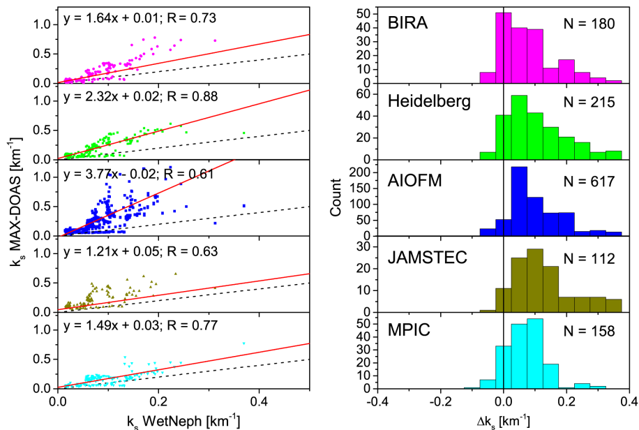
Figure 12. Left panels: correlation between surface extinction from the different workgroups and from WetNeph. The red line shows the linear fit and the dashed line the 1 : 1 line. Right panels: histograms of the difference in surface extinction (MAX-DOAS – WetNeph).
