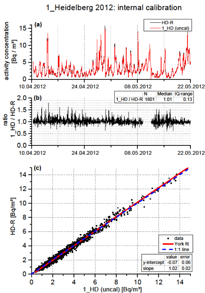
5 Figure 1: Comparison of 214 Po activity concentrations of two Heidelberg Radon Monitors. HD-R is the monitor routinely running at the Heidelberg measurement site. 1_HD (uncal) is a monitor, which had not been calibrated with HD-R before. All monitors that were used for the comparison campaigns were calibrated against HD-R.
