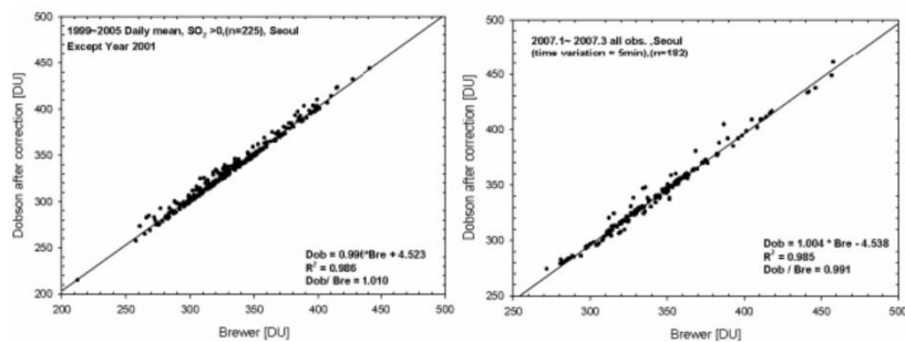
Figure 1. The comparison of Brewer and Dobson measurements in Seoul, Korea. The left figure shows the comparison of Brewer data and Dobson data after SO 2 correction from 1999-2005 except for year 2001 in Seoul. And the right figure shows the same comparison but from January 2007 to March 2007.
