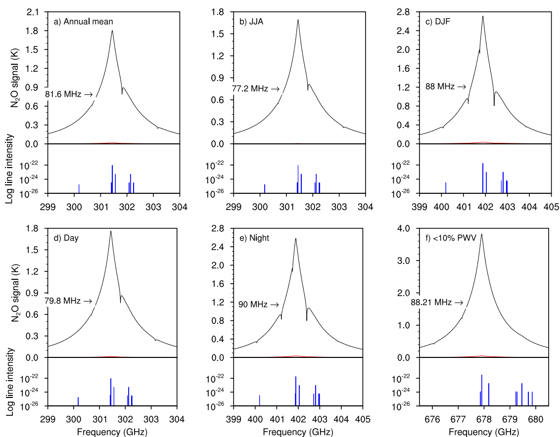
Figure 13. Same as Figure 10 but for \text{N}_2\text{O} . Units of the ordinate scale are K.
