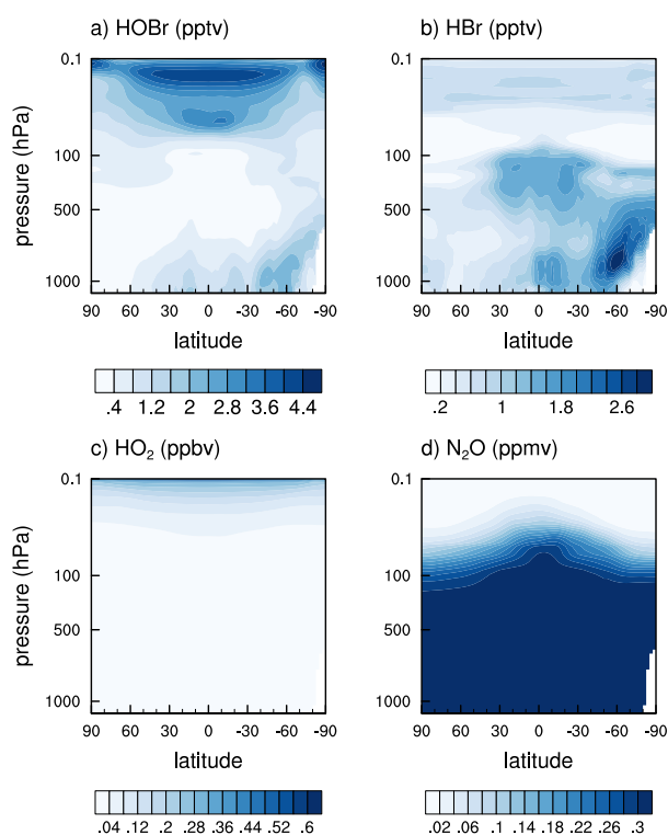
Figure 5. Zonal mean vertical concentrations for a) HOBr, b) HBr, c) HO 2 and d) N 2 O produced by the stratospheric configuration of the UM-UKCA and interpolated to a fixed pressure grid. Data shown are the 2012 annual average. Note the different label bars and units.
