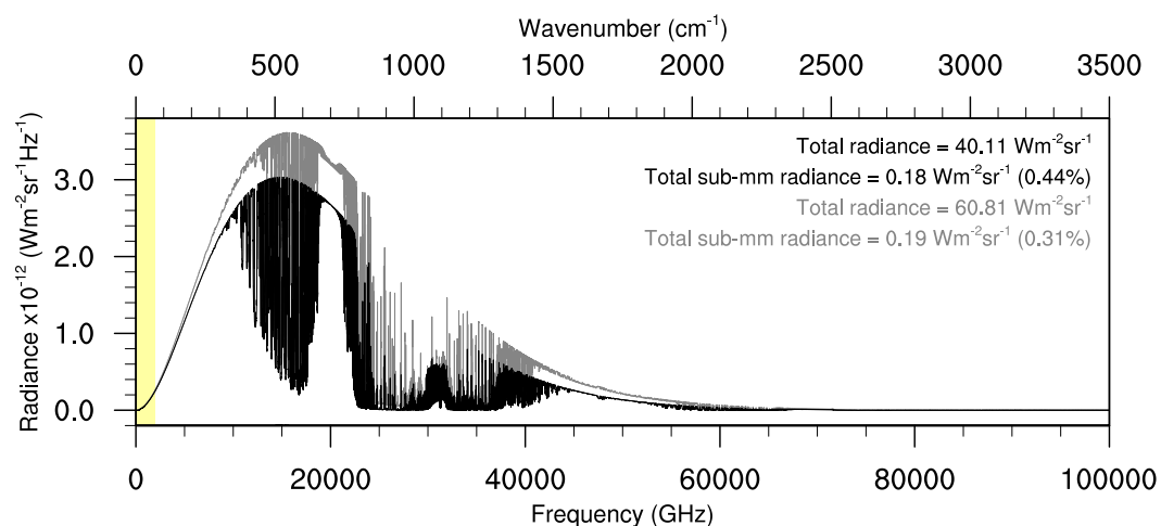
Figure 1. The simulated downwelling spectral radiance (zenith angle = 0^\circ ) received at the Earth's surface over the entire longwave range (1 GHz sampling resolution). The sub-millimetre region (10 - 2000 GHz) is shaded in yellow. Calculations for two polar locations are shown:- a high, dry Arctic case (Summit, Greenland - 3216 m amsl, black) and an Antarctic coastal case just above sea level (Rothera, Antarctica - 16 m amsl, grey). For full details of the simulations see Section 3.
