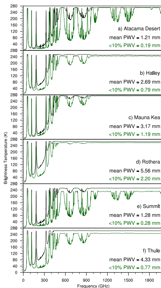
Figure 7. Simulated downwelling brightness temperatures as viewed from the ground for all six locations (a-f). The two scenarios shown are the annual mean (black curve) and the 10% driest profiles (green curve). The mean and the lower decile PWV are shown for each site.
