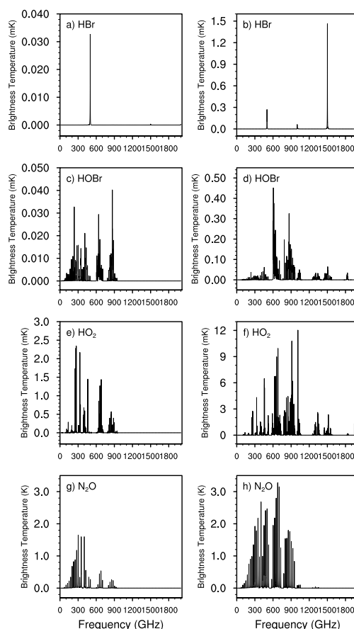
Figure 9. Total frequency range surveys of signal strength for the four species of interest at Summit, calculated as residual brightness temperatures between simulations of the complete atmosphere with and without the species (0.5 GHz sampling resolution). The plots on the left-hand side (a, c, e, and g) are for the annual mean scenario and those on the right-hand side (b, d, f, and h) are for the <10% PWV scenario. Units of the ordinate scale are milliKelvin (mK) except for the \text{N}_2\text{O} plots which are in K. Note the different ordinate scales for each panel.
