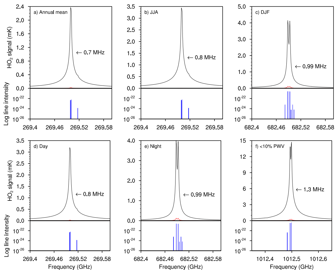
Figure 12. Same as Figure 10 but for \text{HO}_2 .
