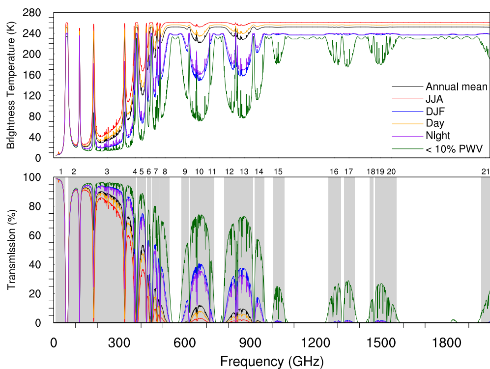
Figure 6. Downwelling brightness temperatures (top), and transmission (bottom) simulated by ARTS for the six scenarios, as viewed from the ground at Summit, Greenland. Window bands (full and partial) are shaded in grey on the lower panel and numbered above. The sampling resolution is 0.5 GHz.
