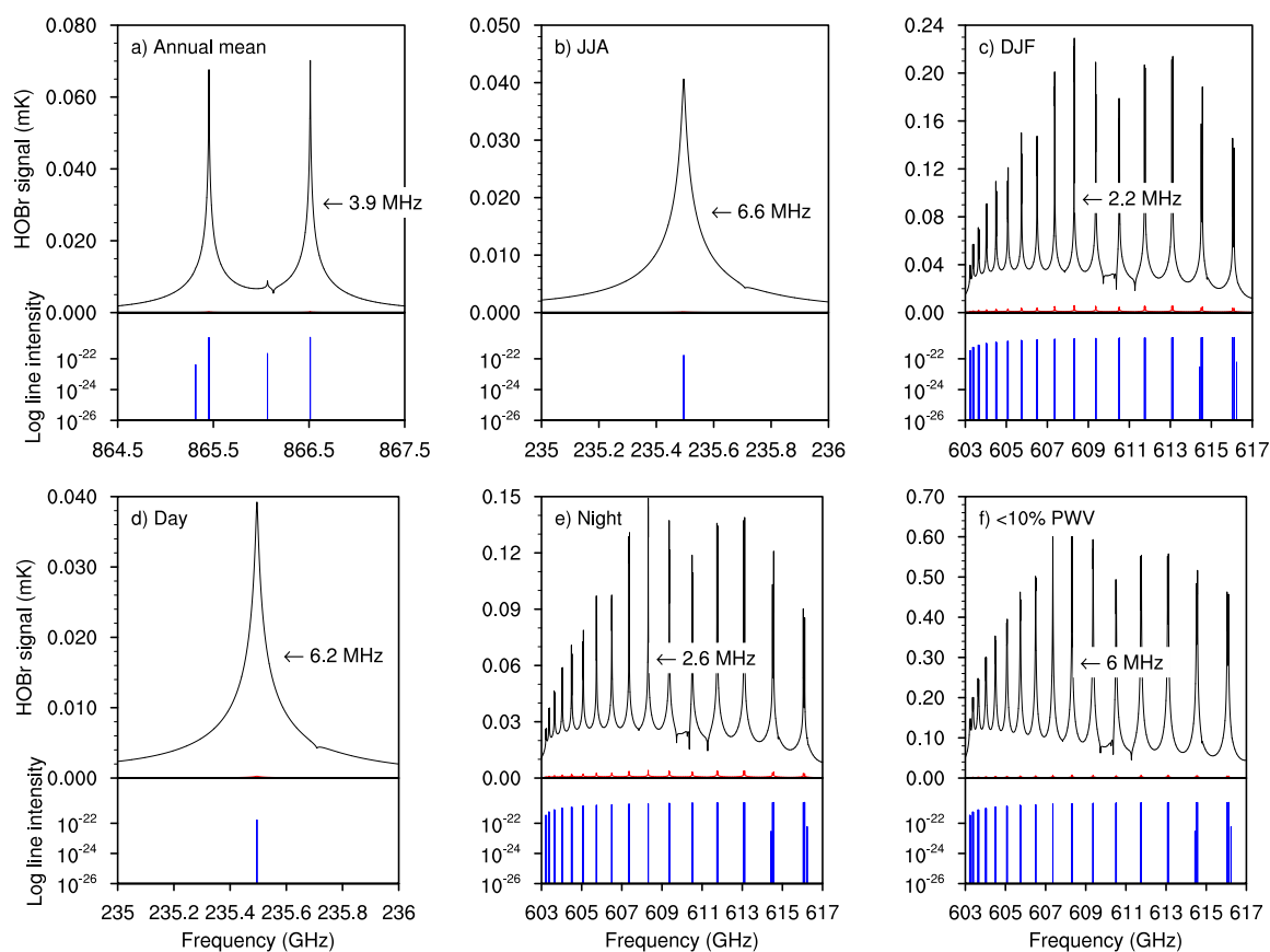
Figure 11. Same as Figure 10 but for HOBr.
