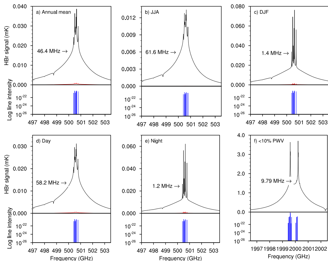
Figure 10. The enhanced HBr signal (1 MHz sampling resolution) around the strongest signal in each scenario (a-f) at Summit, calculated as a residual between simulations with and without HBr. Red lines show the differences that result from using the Ma and Tipping water vapour continuum model. Arrows point to the position of the FWHM of the peak signal in each plot, labelled with the corresponding bandwidth. Units of the ordinate scale are mK. The lower panels in each scenario show HBr intensities taken from the HITRAN database with \log_{10} units of \text{cm}^{-2} (molecule \text{cm}^{-2} ).
