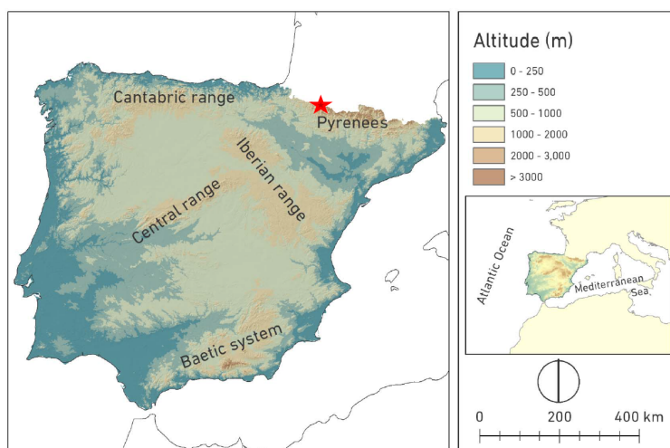
Figure 2. Orography of Spain and location of Formigal-Sarrius site
