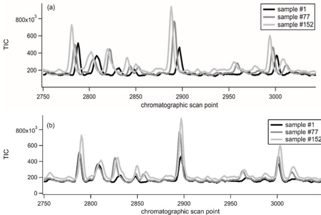
Fig. 1. Figure 2. Excerpts of chromatogram for the 1st, middle and end of the study focus period a) before retention time shift, and b) after retention time shift.
