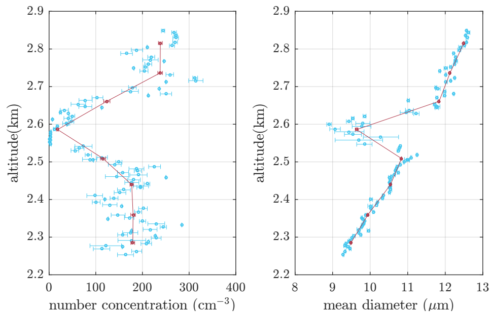
Fig. 3. Comparison of two vertical profiles for the cloud droplet number concentration (left) and mean cloud droplet diameter (right) for the run at 13:31 on February 2015.
