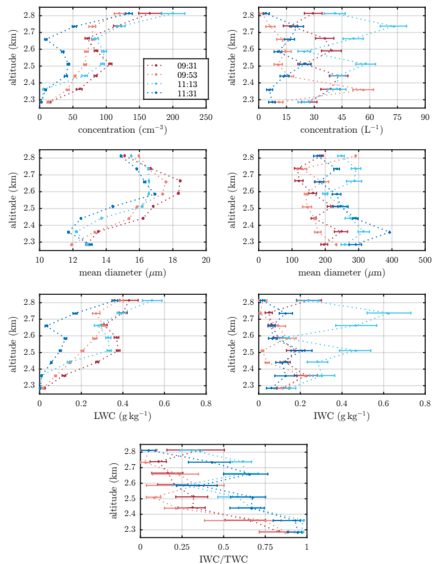
Fig. 4. Height profiles of the cloud droplet and ice crystal number concentration, mean diameter and water content (LWC and IWC) and the ratio of the ice water content to total water content (IWC/TWC) on 21 M
