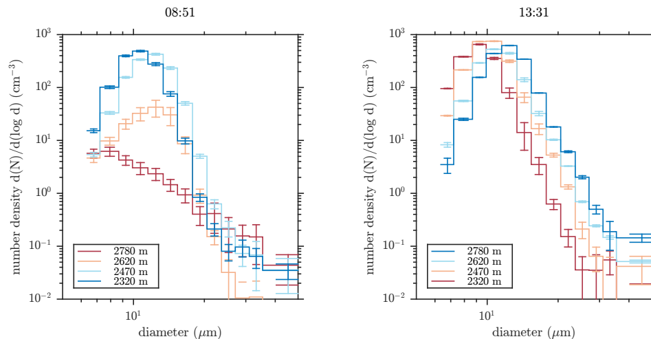
Fig. 2. Height resolved cloud droplet size distribution during the 8:51 run in the morning (left) and the 13:31 run in the afternoon (right).
