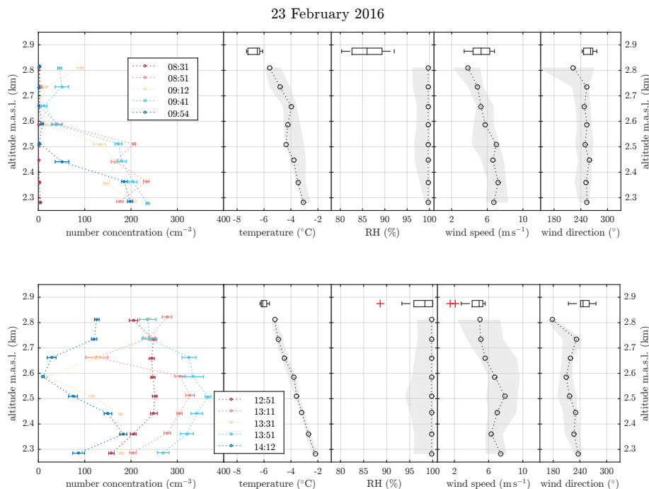
Fig. 1. Height profiles of the Liquid Case measured with the HoloGondel platform during the morning (top) and the afternoon (bottom) of 23 February 2016. The data is averaged over an altitude interval of 75m.
