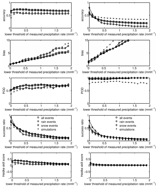
Fig. 1. Figure 4. Accuracy, bias score, hit POD, success ratio and Heidke skill score (from top to bottom) against precipitation measurements for the period 1995-1997 (left HOAPS, right ERA-Interim) as a function
