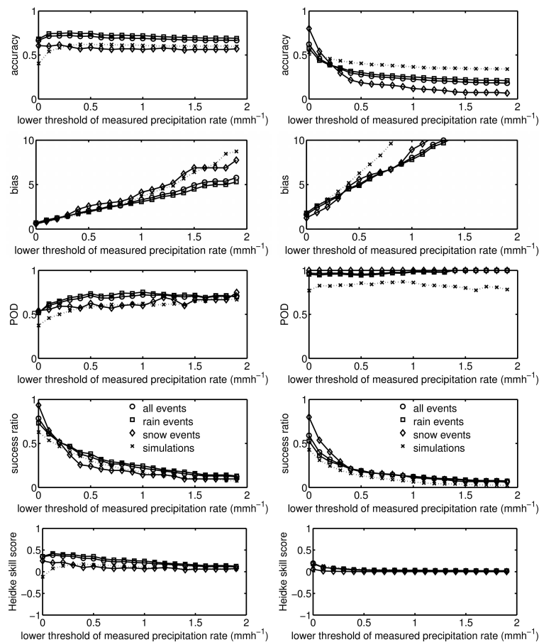
Fig. 1. Figure 4. Accuracy, bias score, hit POD, success ratio and Heidke skill score (from top to bottom) against precipitation measurements for the period 1995-1997 (left HOAPS, right ERA-Interim) as a func
