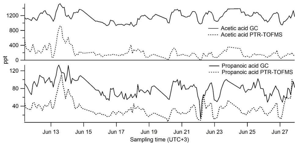
Fig. 3. Comparison of mixing ratios (pptv) measured by GC-MS and PTR-TOFMS at SMEAR II in June 2015.
