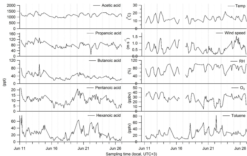
Fig. 1. Mixing ratios (pptv) of volatile organic acids (C 2 -C 6 ) and trace gases together with meteorological parameters at SMEAR II station in Hyytiälä, Finland.
