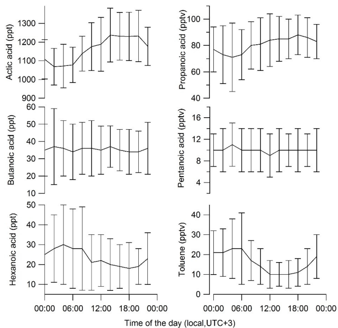
Fig. 2. Mean diurnal variation of the mixing ratios with standard deviations (error bars) at SMEAR II between 11 and 27 June 2015.
