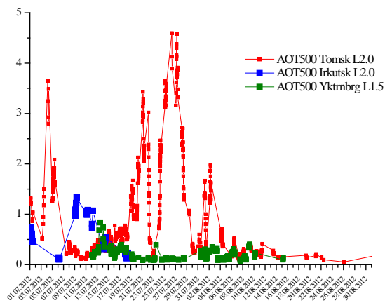
Figure 1. Time variations in atmospheric AOD ( 0.5 \mu\text{m} ) at three AERONET stations in the Siberian region (July-August 2012)
