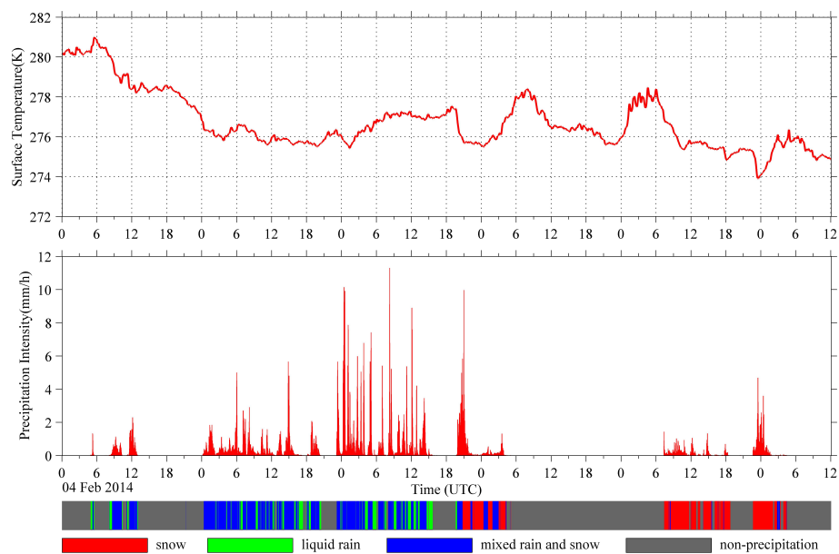
Fig. 2. precipitation intensity and types
