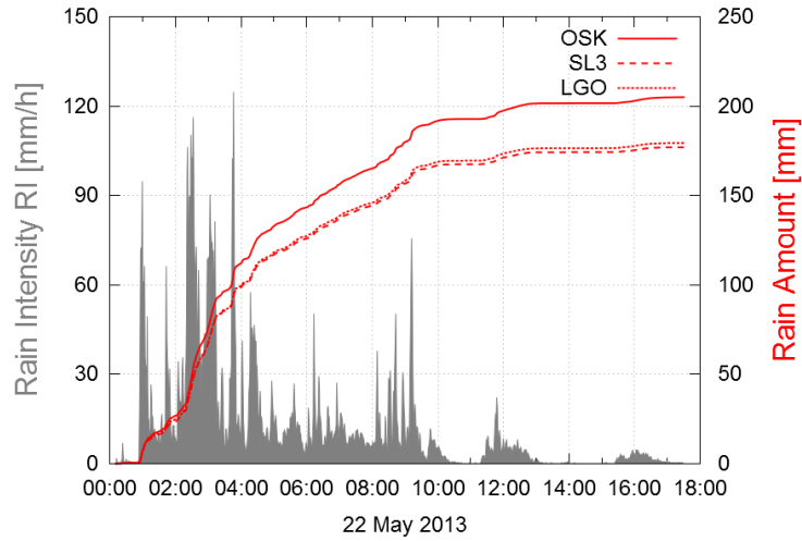
Figure 3. Reference rainfall intensity measured by the OSK drop counter (shaded gray background) and comparison of the accumulated reference (red continuous line) with the accumulated Logotronic (LGO) and Shanghai (SL3) measurements during the sample event of 22 May 2013.
