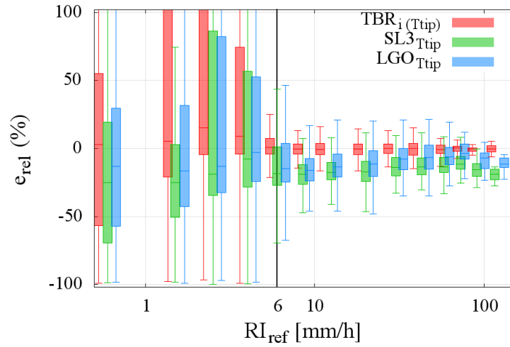
Figure 5. One-minute relative deviations ( e_{rel} ) between the three TBRGs (including the ideal one) and the reference (OSK) when adopting the inter-tip post-processing algorithm (Tip).
