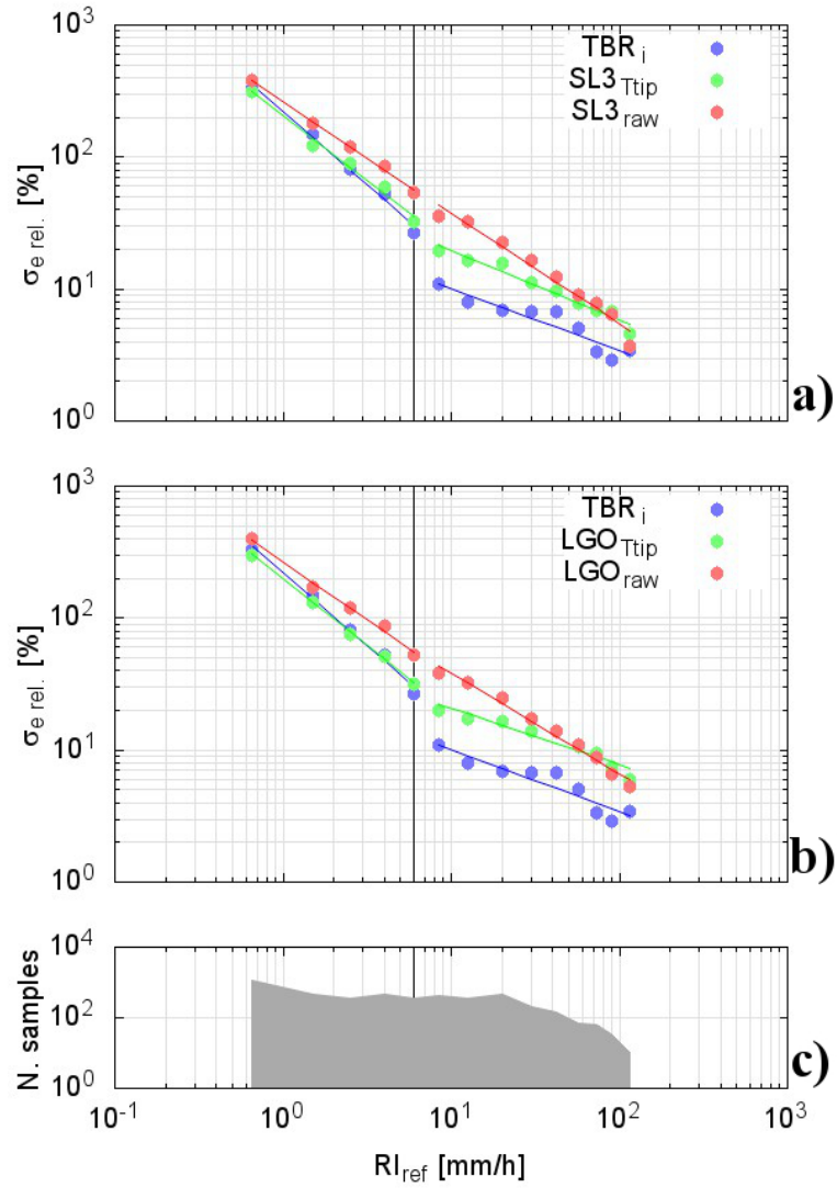
Figure 8. Standard deviation of the relative error for the ideal and the investigated TBRGs when adopting the inter-tip time algorithm (Ttip) and the tip counting method (raw) with respect to the ideal gauge for both the SL3 (a) ad LGO (b) instruments. In panel (c) the sample size for each RI class is reported.
