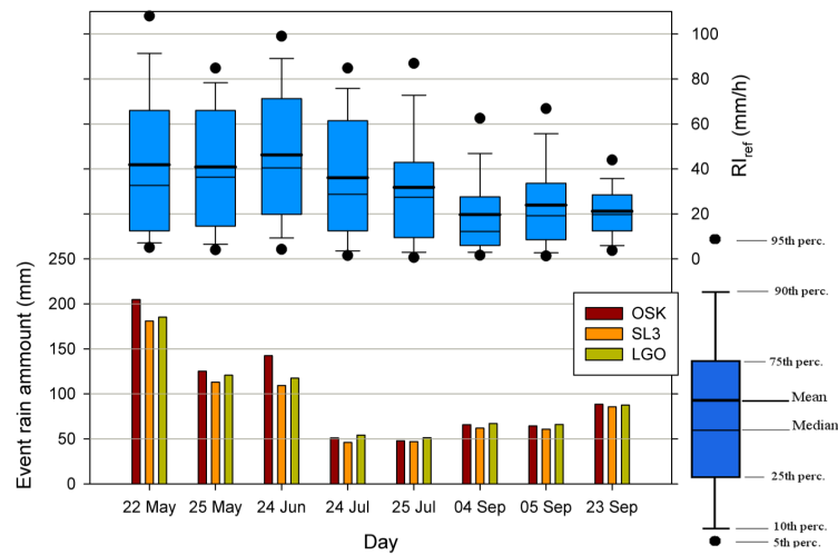
Figure 4. Box plot of the reference rainfall intensity for each event (top of the graph) and corresponding daily rain amount (lower part of the graph) for the OSK drop counter (reference) and the two TBRGs (SL3 and LGO). The explanation of the symbols used in the box-plot representation is shown on the right side of the graph.
