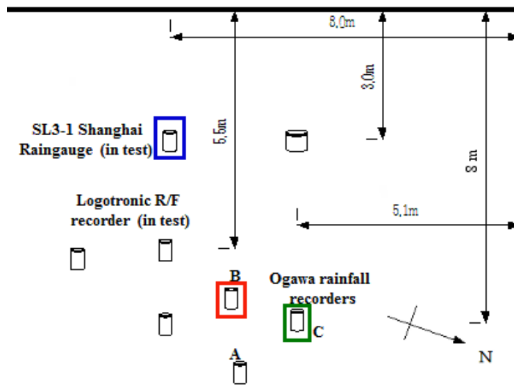
Figure 2. The West corner of the Hong Kong Observatory field test site where the SL3 (blue box), the LGO (red box) and the OSK (green box) are located. The distance of each instrument from the field site borders is indicated.
