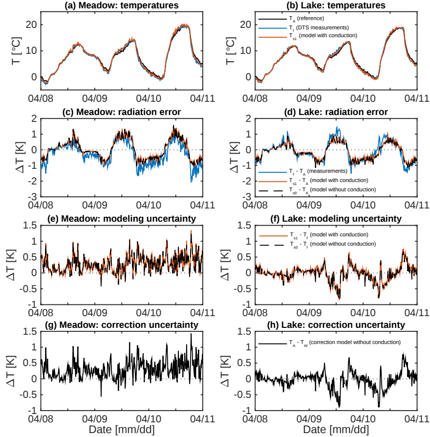
Figure 5. Comparison of measured and modeled temperatures ( 10 min averages ) from 8 to 10 April 2015 (mostly clear sky) at 2.00 and 2.13 m height above the meadow and the lake respectively: a,b Fiber ( T_f , T_{s1} ) and reference air temperatures ( T_A ). c,d Radiation error: fiber minus air temperature. e,f Modeling uncertainty: modeled minus measured fiber temperature. g,h Correction uncertainty: reference air minus corrected fiber temperature. In this figure, T_{s1} depicts fiber temperatures modeled with high thermal conductivity ( 0.6 \text{ J s}^{-1} \text{ m}^{-1} \text{ K}^{-1} ) but there was no difference to model versions with low conductivity or without conduction. On 9 April, 15:50 – 16:10 local standard time (LST) there was a data gap in the DTS measurements resulting from an interruption when splicing to fix a fiber break.
