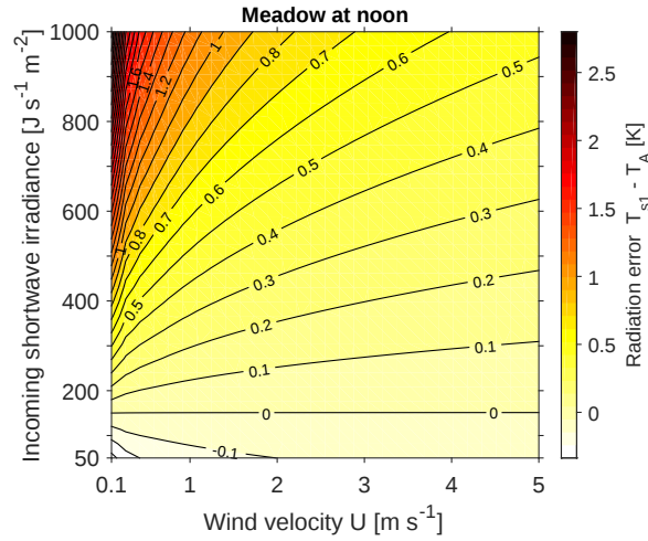
Figure 6. Radiation error T_{s1} - T_A as function of the main drivers total incoming shortwave irradiance on a horizontal surface and wind velocity. The model predictions for 2 m height above meadow were based on conditions from 10 April 2015, 12:00 LST with an air temperature of 16.8 °C, a sun elevation of 53 °, a fixed ratio of direct to total shortwave irradiance of 0.91 and a net longwave radiation of 117 J s -1 m -2 . Incoming shortwave irradiance and wind velocity were initially 724 J s -1 m -2 and 0.26 m s -1 respectively. Reflected shortwave irradiance was calculated by multiplying the incoming shortwave irradiance with the albedo of the meadow given by the initial ratio of reflected to incoming shortwave irradiance (0.22). Here, only the results for low thermal conductivity (0.1 J s -1 m -1 K -1 ) of fabric and fiber are shown as the results for high thermal conductivity (0.6 J s -1 m -1 K -1 ) were similar.
