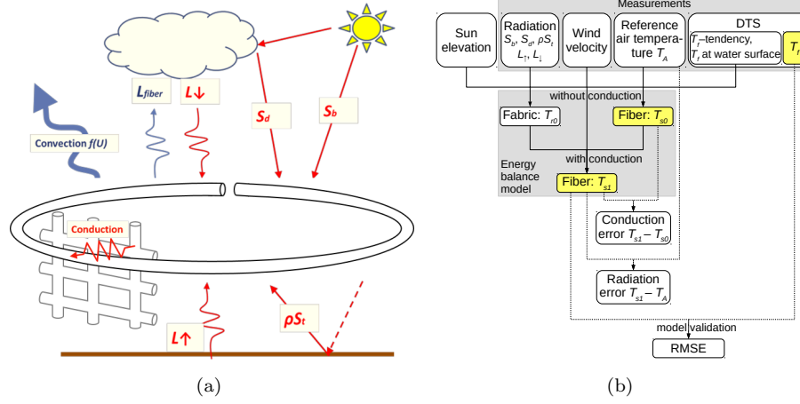
Figure 4. a Incoming (red) and outgoing (blue) energy balance components for a fiber coil (adapted from Sayde et al. , 2015). S_b , S_d and \rho S_r are direct, diffuse and reflected shortwave radiation respectively, L_{\downarrow} and L_{\uparrow} are downward and upward longwave radiation respectively and L_{fiber} is longwave radiation emitted by the fiber coil. Conduction results from temperature differences between fiber coil and reinforcing fabric. b Flow chart of error estimation for the DTS columns with a proposed energy balance model. T_f is the measured fiber temperature whereas T_{s0} and T_{s1} are modeled fiber temperatures. RMSE denotes Root Mean Square Error.
