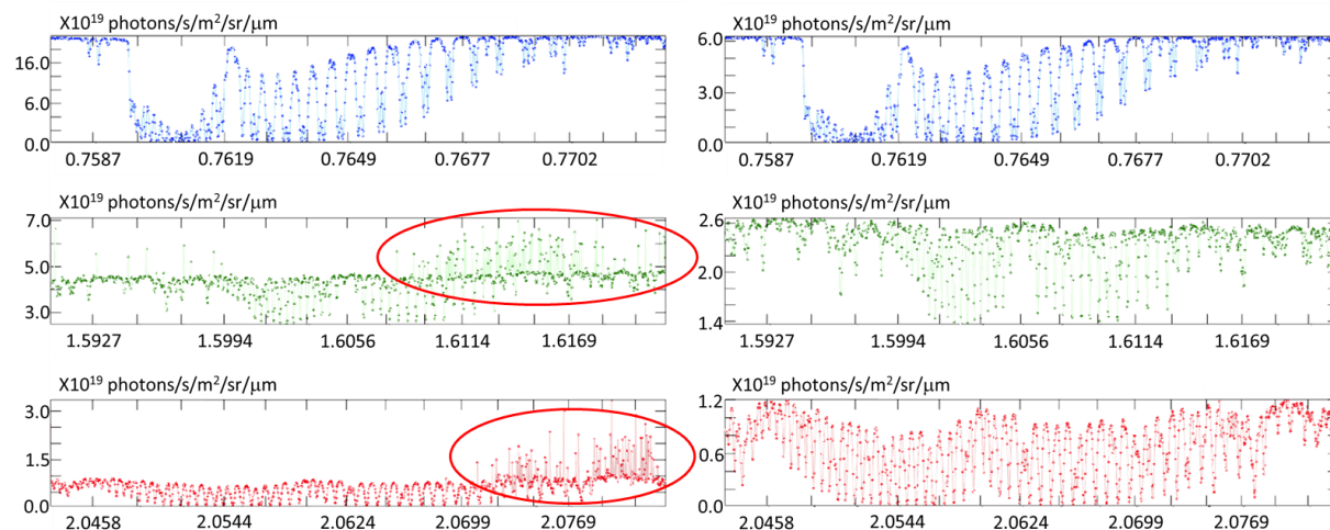
Figure 8: Spectra recorded in footprint 3 of the ABO2 (top), WCO2 (middle) and SCO2 (bottom) channels on August 8 (left) and September 10 (right) show the impact of an improved dark calibration. The August 8 spectra were calibrated using FPA dark response recorded during the pre-launch thermo-vacuum tests at JPL in 2012. The September 10 spectra were calibrated using dark data recorded in flight. The revised dark data and bad pixel maps dramatically improve the quality of the spectra at longer wavelengths in the WCO2 and SCO2 channels.
