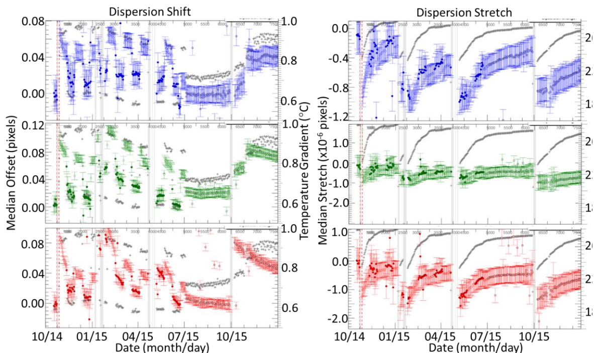
Figure 7: The time evolution of the dispersion shift/offset (left column) and dispersion stretch (right column) are shown for the ABO2 (top, blue symbols), WCO2 (middle, green symbols) and SCO2 (bottom, red symbols) channels. Both are shown on the left hand ordinate of each plot. The shifts are expressed in pixels, while the stretch is expressed as a ratio with the fixed dispersion stretch term, subtracted from 1, in parts per million. The shifts are well correlated with temperature gradients across the OBA (dark grey crosses and right hand ordinate), which can introduce grading tilts and other distortions in the OBA. The stretch term is correlated with the cryocooler temperature (dark grey symbols and right hand ordinate). These shifts appear to be correlated with time between Decon cycles, indicated as vertical grey bars.
