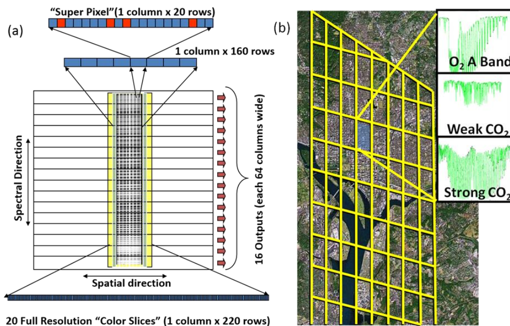
Figure 2: The illumination and readout approach used for the OCO-2 FPAs, showing the direction of spectral dispersion from bottom to top, and the spatial direction from left to right. The ~160 illuminated pixels in the spatial dimension are summed into eight 20-pixel “footprints.” If one or more of the pixels in a footprint is “bad” (red pixels), it is eliminated from the sum. If one or two contiguous pixels in a column are bad, then they are replaced with the average of their good neighbors. If three or more bad pixels are contiguous, then they are replaced with zeros. This algorithm is only applied in the spatial direction—spectral information is never mixed. One of the 20 full-resolution “color slices” is also shown at the bottom. (b) Spatial layout of 8 cross-track footprints for nadir observations over Washington, D.C. Each footprint is shaped like a parallelogram, rather than a square, because of the rolling readout of the FPAs and the spacecraft motion.
