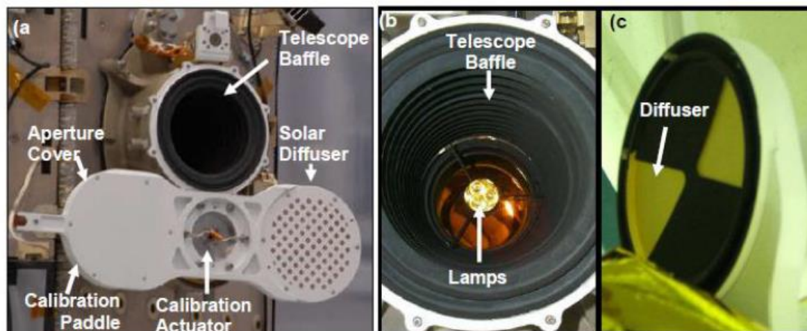
Figure 3: The On-board Calibrator (OBC) is attached to the telescope baffle assembly. (a) The OBC is shown in the “open” position for taking science data, with the aperture cover is to the left and the solar diffuser to the right. (b) The telescope baffle assembly is shown along with the incandescent lamps used to illuminate the diffuser on the back of the aperture cover. (c) The inner surface of the aperture cover is partially coated with a roughened gold surface that is illuminated by the lamps to produce a spatially uniform illumination field.
