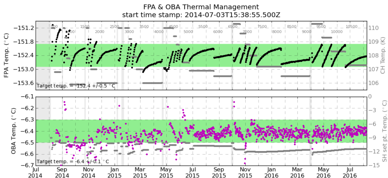
Figure 4: Thermal performance of the OCO-2 instrument FPAs (top) and OBA (bottom) are shown as a function of time for normal operations. The FPA temperatures (black dots in top plot) are maintained by controlling the temperature of the cold head (CH) of the cryocooler. The CH temperatures are shown as grey points (that appear as horizontal grey lines) in the top plot, and their values are labeled on the right hand y-axis. During routine operations, the CH temperatures must be adjusted as ice accumulates on the thermal blankets that insulate the thermal straps linking the FPAs to the CH, reducing their efficiency. OBA temperatures (pink dots in bottom plot) are maintained by controlling the temperature of the thermal shroud that encloses the OBA. The set point of the shroud (SH set pt.) is shown as grey points on the bottom plot and their values are labeled on the right hand y-axis of that plot. The light grey vertical bars indicate decontamination cycles when normal operations are suspended and the FPAs and OBA are raised to near room temperature to remove ice from the thermal straps and FPAs.
