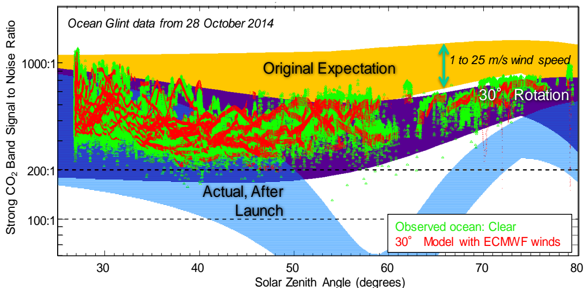
Figure 17: The continuum signal to noise ratio (SNR) for ocean glint observations is shown as a function of solar zenith for the SCO 2 channel. The gold band shows the performance originally predicted using a Cox-Munk ocean reflectance model for wind speeds varying from 1 to 25 m/sec. The actual performance observed immediately after launch, when the spectrometer slits were oriented perpendicular to the principal plane, fell within the light blue band. The low values between 50 and 60° are near the Brewster angle. Predictions from the Cox-Munk ocean reflectance model indicated that introducing a 30° yaw around the center of the instrument's field of view would yield values within the purple band (actual predictions shown as red points). After this change in the observing geometry was implemented, the observed SNR for clear-sky ocean soundings increased to values above 200:1 at most solar zenith angles (green points). The SNR in the other two channels is somewhat higher because the solar flux is larger there.
