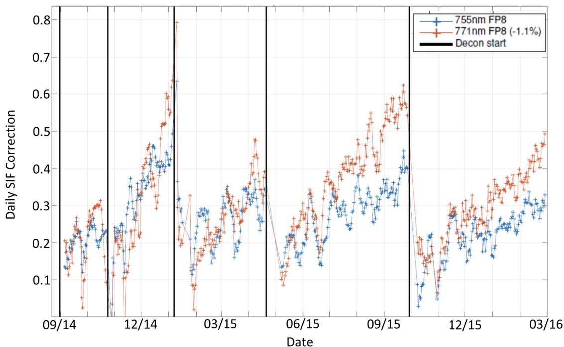
Figure 19: The correction applied to the Solar Induced Chlorophyll Fluorescence (SIF) estimate is shown as a function of time for the solar lines located near 755 (blue) and 771 nm. The timing of the decon activities is indicated by the vertical black lines. These observations suggest that as ice accumulates on the ABO2 FPA, increasing its reflectance, a fraction of that light may be scattered back to the FPA by the cold filter, and other optics above the FPA, producing a zero level offset.
