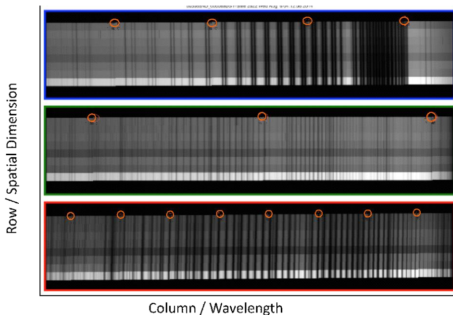
Figure 12: Images of the ABO2 (top), WCO2 (middle) and SCO2 (bottom) channels in “summed mode” taken from the OCO-2 first light frame over Papua New Guinea. The 8 spatially-summed footprints in each band are shown from bottom (footprint 1) to top (footprint 8). In this 0.333 second frame, footprint 1 was contaminated by a cloud and appears brighter than the rest. This frame clearly shows the rotation, or “clocking” of each FPA columns with respect to the dark O 2 and CO 2 absorption lines. The O 2 lines are tilted slightly counter-clockwise, while the CO 2 lines in the WCO 2 and SCO 2 channels are tilted clockwise. The columns where the 1-pixel clocking adjustments are applied are highlighted with red circles.
