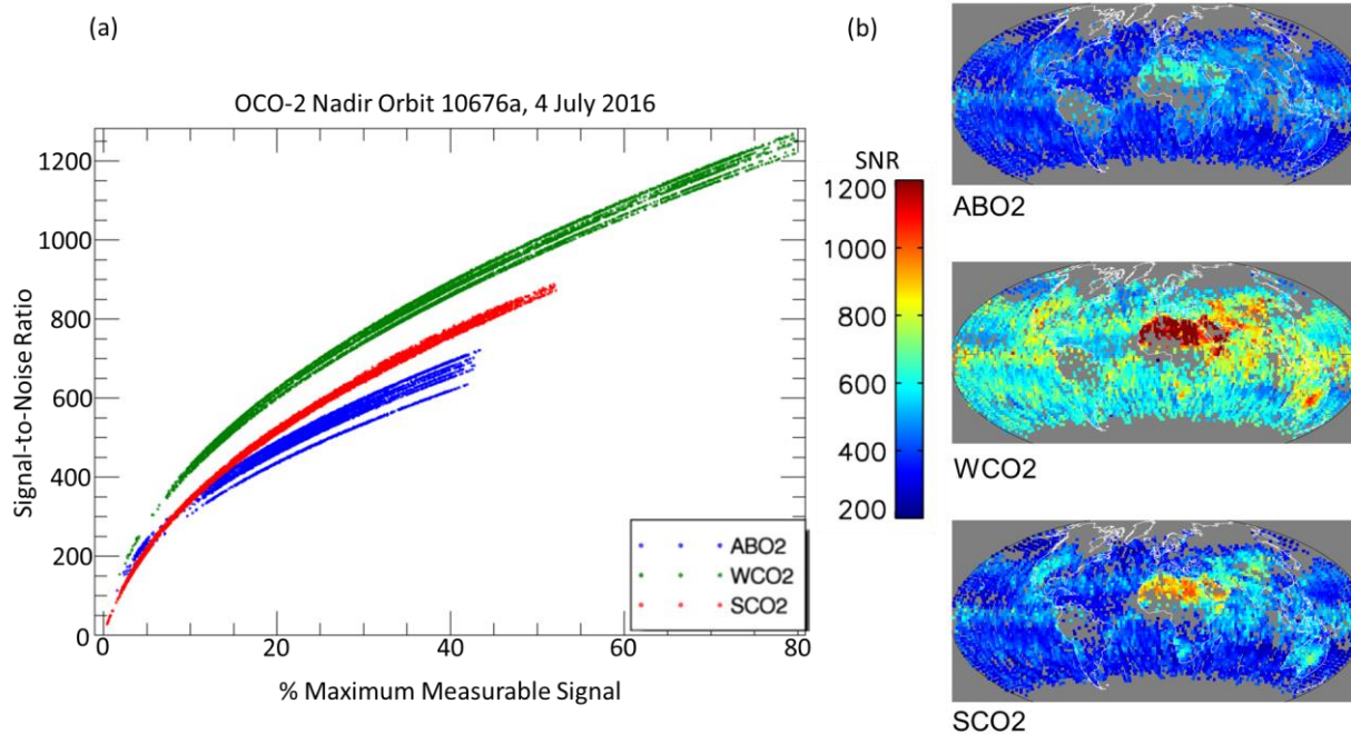
Figure 5: (a) Median Signal-to-Noise Ratios (SNR) for individual soundings in the ABO2 (blue), WCO2 (green), and SCO2 (red) channels are shown as a function of the % maximum measurable signal for a nadir orbit observed on 4 July 2016. The parallel traces show results for the 8 footprints in each channel. (b) The mean continuum single-sounding signal-to-noise ratios (SNR) in 2^\circ \times 2^\circ bins is shown for the ABO2 (top), WCO2 (middle), and SCO2 (bottom) channels for April 2015.
