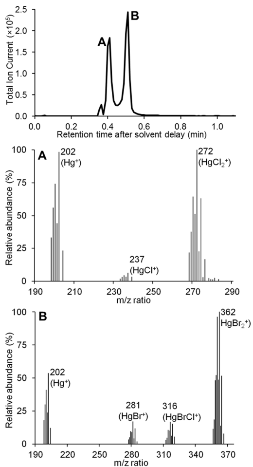
Figure 2. Chromatogram of a mixed standard of \text{HgCl}_2 and \text{HgBr}_2 in acetone ( 0.5 \mu\text{g } \mu\text{L}^{-1} for each compound) (top), mass spectra for \text{HgCl}_2 (A, middle) and \text{HgBr}_2 (B, bottom). Solvent delay was 2 min.
