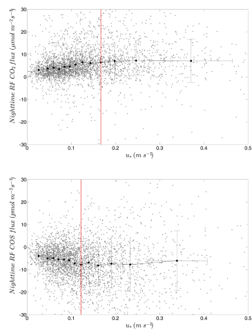
Figure R2.2 U^* thresholds (red vertical lines) determined with the change-point-detection after Barr et al. (2013).
