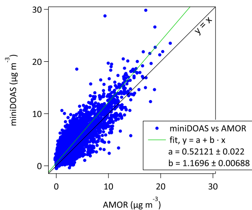
Figure 10: Scatter plot (8130 data points) of hourly ammonia concentrations measured at the monitoring station in De Zilk for 1 September 2014 up to and including 31 December 2015. The fit shown is a least orthogonal distance fit.
