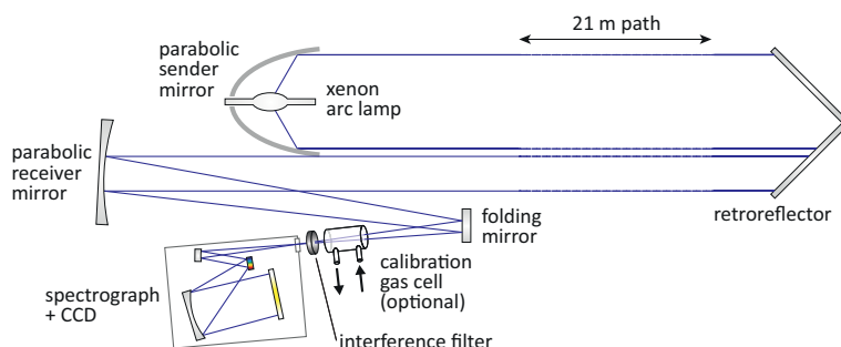
5 Figure 2: Schematic representation of the miniDOAS, with an optional calibration gas cell in the optical path.
