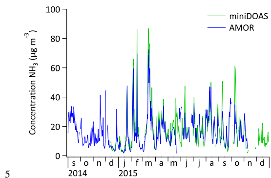
Figure 11: Daily ammonia concentrations measured at the monitoring station in Vredepeel for 1 September 2014 up to and including 31 December 2015.
