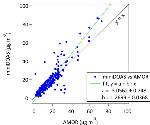
Figure 12: Scatter plot (259 data points) of daily ammonia concentrations measured at the monitoring station in Vredepeel for 1 September 2014 up to and including 31 December 2015. The fit shown is a least orthogonal distance fit.
