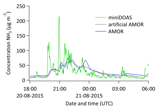
Figure 7: Vredepeel, miniDOAS minute data converted to artificial AMOR data by delaying and smoothing. Here we used an e-folding time \tau_{1e} of an hour. The delayed and smoothed miniDOAS data becomes remarkably similar to the AMOR data. Note that the surfaces under the various curves are more or less similar, indicating that both instruments on average detect similar amounts of ammonia.
