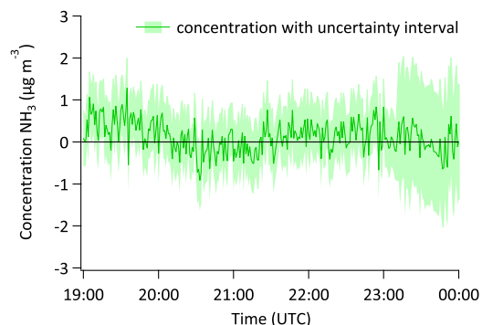
Figure 4: Example of an episode of very low ambient ammonia concentrations, as measured with the miniDOAS at Wieringerwerf on 16 August 2015. Minute values of the measured ammonia concentrations in \mu\text{g m}^{-3} are indicated by a green line, the light green area around this line indicates the 1-sigma uncertainty interval.
