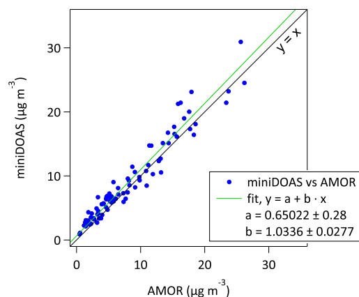
Figure 14: Scatter plot (89 data points, R^2=0.94 ) of monthly ammonia concentrations measured at all stations combined for 1 September 2014 up to and including 31 December 2015. The fit shown is a least orthogonal distance fit.
