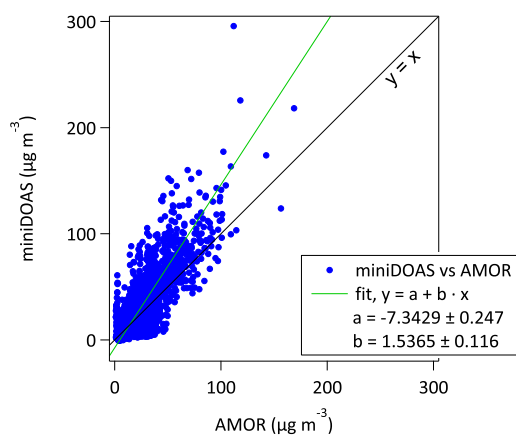
Figure 9: Scatter plot (6429 data points) of hourly ammonia concentrations measured at the monitoring station in Vredepeel for 1 September 2014 up to and including 31 December 2015. The fit shown is a least orthogonal distance fit.
