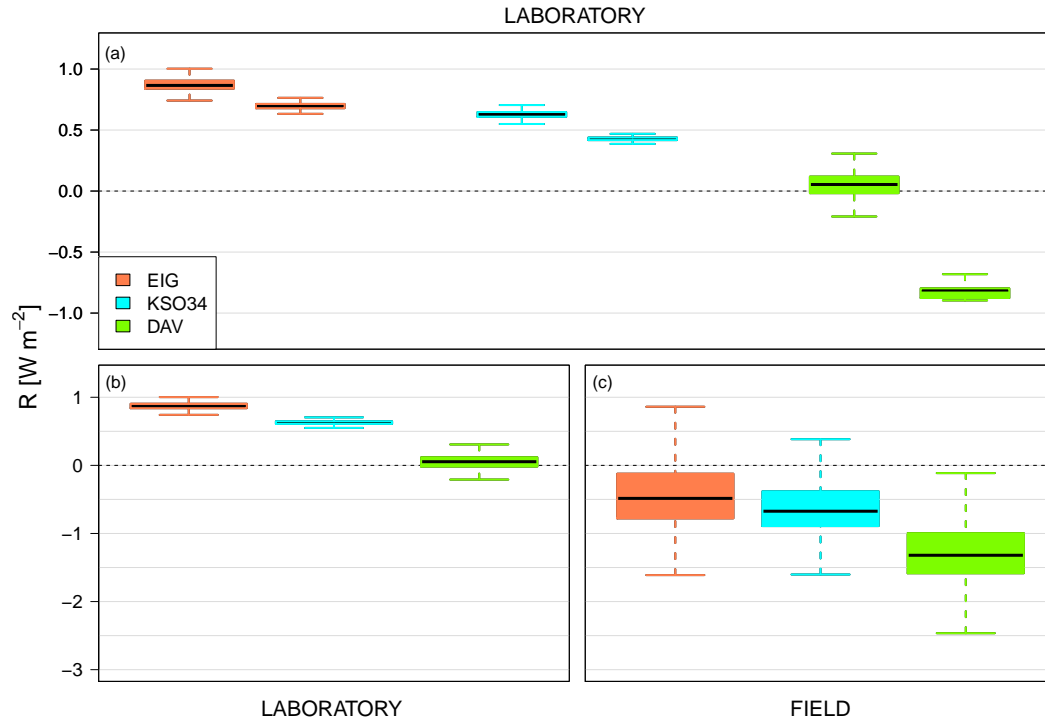
Figure 3. Spread of radiation measurements ( R ) with CMP21 pyranometers contained in different HV-systems (EIG, KSO34 and DAV) during dormant (i.e., undisturbed) phases during (a) and (b) laboratory and (c) field campaigns. Panel (a) provides results for two CMP21 pyranometers per HV-system as multiple instruments have been available during the laboratory campaign.
