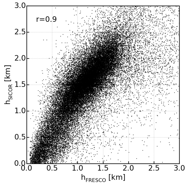
Figure 1. Scatter plot of the retrieved cloud height h_{\text{SICOR}} in km with the one provided by Fresco h_{\text{FRESKO}} . For the year 2003 over the ocean in the latitude/longitude box [(30^\circ\text{S}, 30^\circ\text{W}), (0^\circ, 0^\circ)] with cloud optical thickness > 1 are shown.
