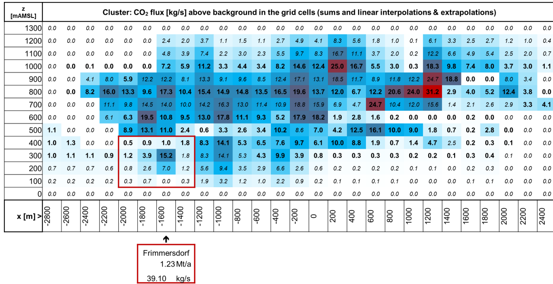
Figure 7. The same as Fig. 4, however for the mixed plume of the whole cluster on the northern transect. The weak plume from Frimmersdorf, which is only 4 km away from this cross section could be isolated below 450 mAMSL. The confirmation was done with an analysis with higher resolution. The layer between 350 and 450 m (centered at 400 m) has enough measurement points allowing to separate the small lower plume from the main plume from Niederaußem (probably the whole width of about 4.5 km) and the two plumes from Neurath old and new. See Fig. 8 for the separation on a cross section upwind of Frimmersdorf, closer to the three other plumes.
