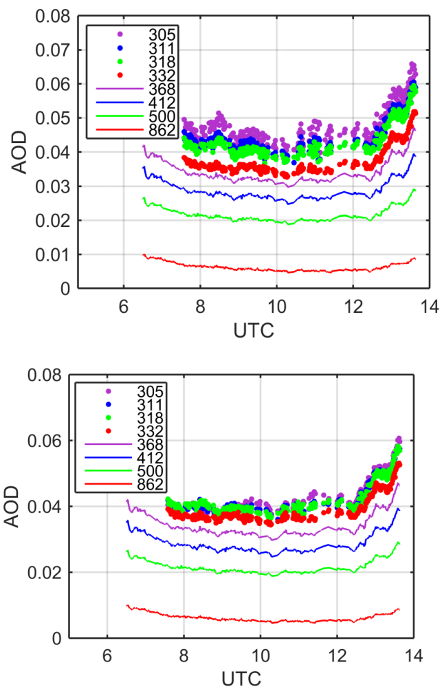
5 | Figure S4: 1-minute AOD determined by UVPFR #1001 (dots) and PFR-N24 (lines) on the 12th October 2015 in Davos. Data points disturbed by clouds have been removed.
