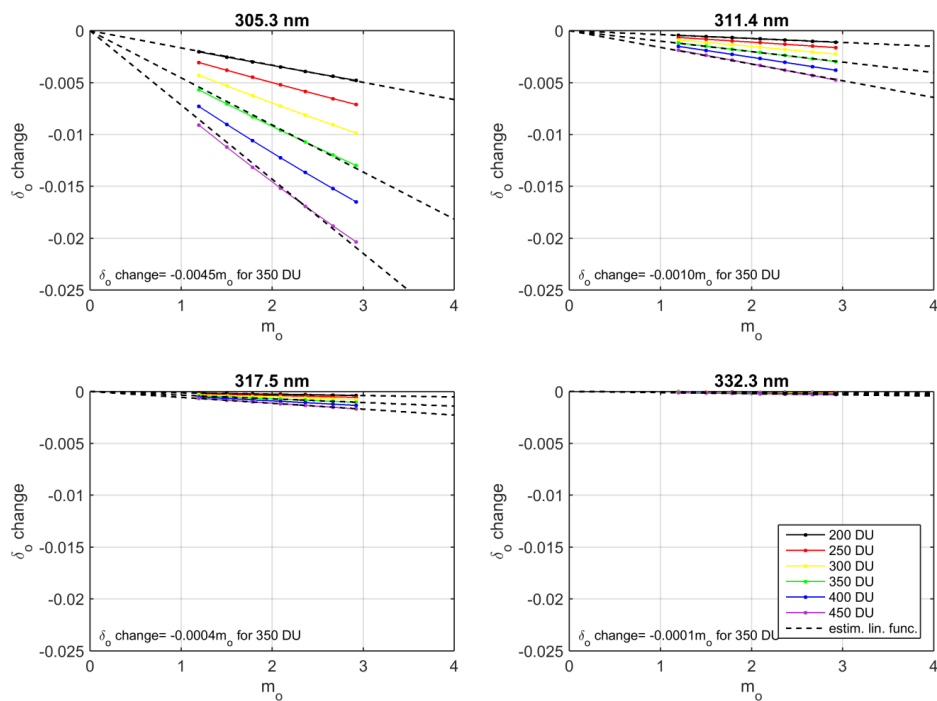
Figure 2: Calculated change in effective ozone optical depth with airmass due to the UVFPR filter bandwidths.
