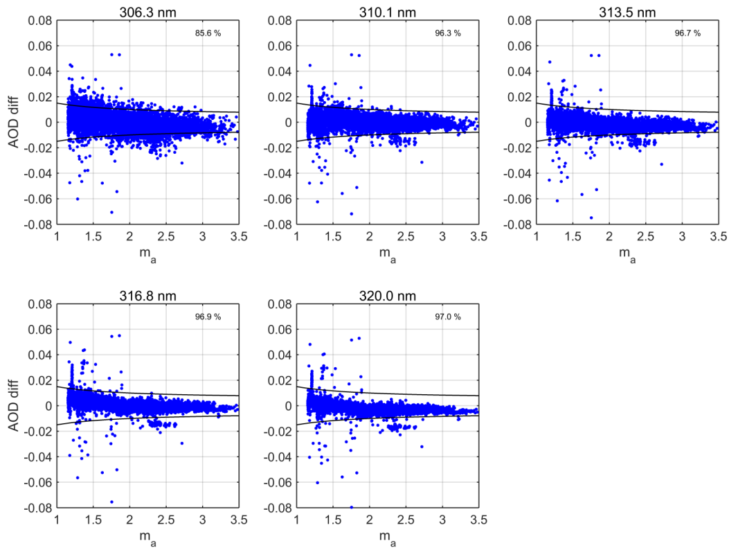
Figure 76: Differences in AOD, UVPFR-Brewer, at Brewer wavelengths for measurements during autumn 2015 and spring 2016 in Davos. Percentage of differences within WMO traceability limits is given in each graph.
