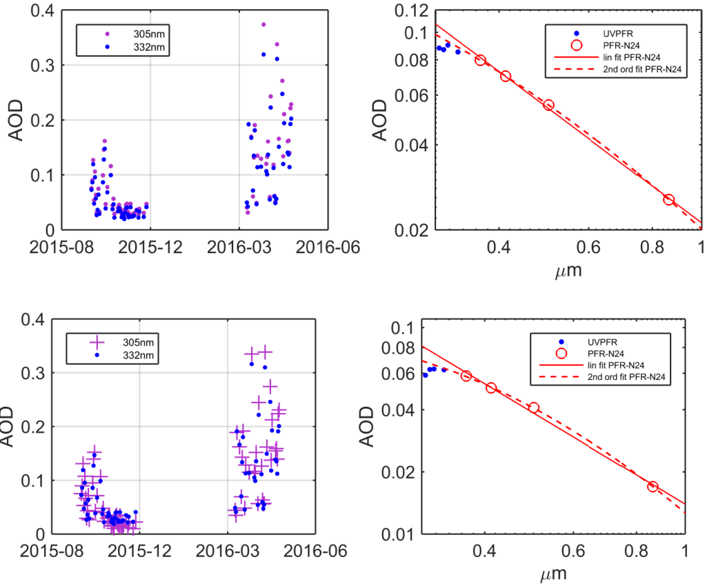
5 Figure 65: Daily mean AOD at 305 and 332 nm in Davos (left) and mean of daily means of AOD during the whole study from the UVPFR and a standard PFR (right).
