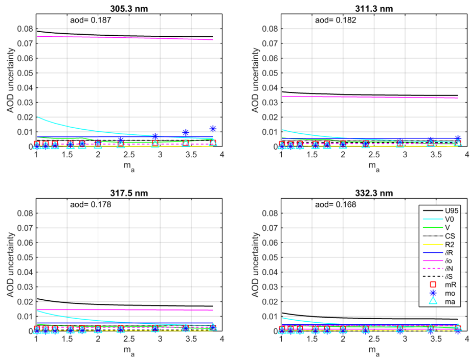
Figure 43: Estimated expanded uncertainties, k=2 , (black lines) of AOD for the UVPFR #1001 wavelengths. Individual contributing uncertainties sources, at an approximate level of confidence of 95 %, are also shown. Calculations are made for a day 2 months after a calibration and with total column ozone amount of 350 DU.
