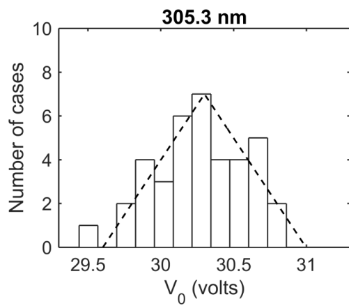
Figure 3. Frequency distribution of V_0 for the 305 nm channel derived with the refined Langley plot method (Eq. 3) during both calibration periods 2015 and 2016 at Izaña. The results were approximated with a triangular distribution indicated by the dashed line.
