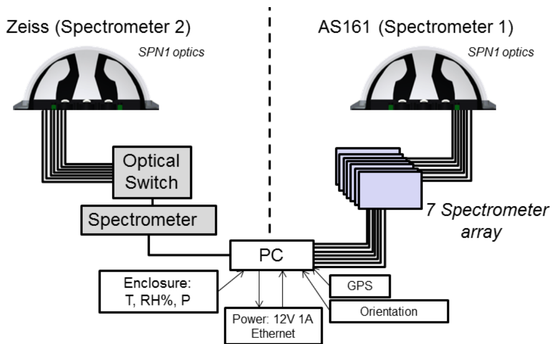
Figure 2: System diagram for the two spectrometer configurations. Elements in white are common to both configurations, although each have their own separate PC, GPS etc. Main configurational difference is that the AS161 (Spectrometer 1) contains seven spectrometers, whereas the Zeiss (Spectrometer 2) contains only one which is connected to the seven optical channels via an optical switch. The PC enclosure temperature (T), relative humidity (RH) as well as atmospheric pressure (P) is monitored.
