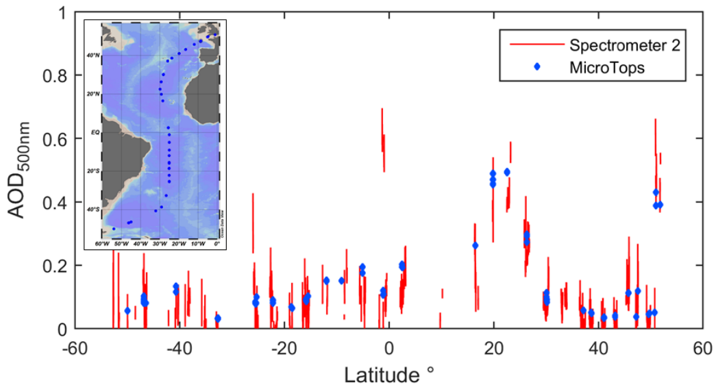
Figure 14: General evolution of AOD 500nm as measured by Spectrometer 2 (Zeiss, red line) and MicroTops (blue diamonds) over the duration of the AMT24 cruise. Map of the MicroTops sampling locations shown in upper left of figure.
