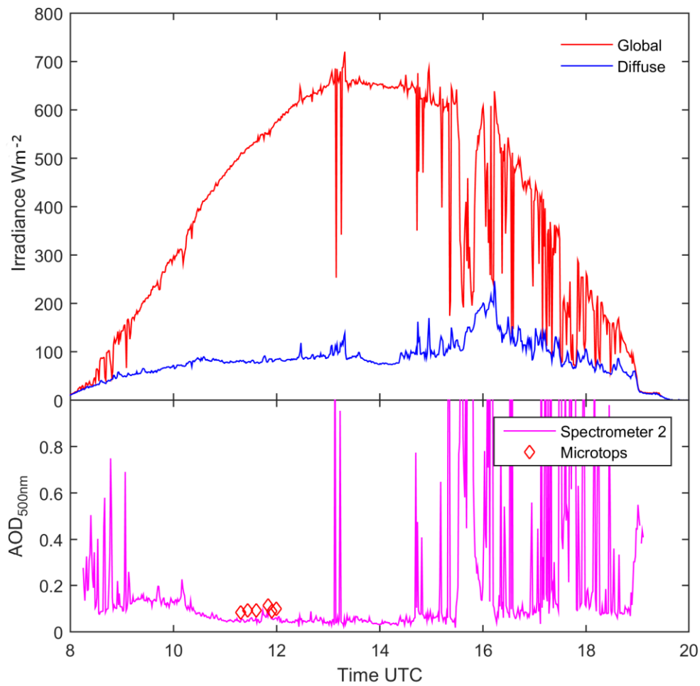
Figure 10: Time-series plots of integrated PAR values of I_G and I_D (upper plot) and AOD_{500nm} (lower plot) for 4 October 2014. The Microtops 500nm values are superimposed on the AOD plot. Cloud affected AOD have not been removed from the spectrometer database.
