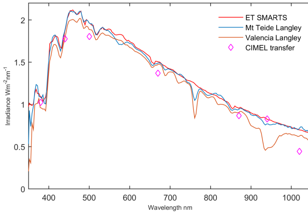
Figure 4: Calibration curve for Spectrometer 2 (Zeiss). Extra-terrestrial spectrum as predicted from the SMARTS2 model, Langley calibrations on Mt Teide (Tenerife), Valencia (Spain), and from calibration transfer from the CIMEL sun photometer at Valencia.
