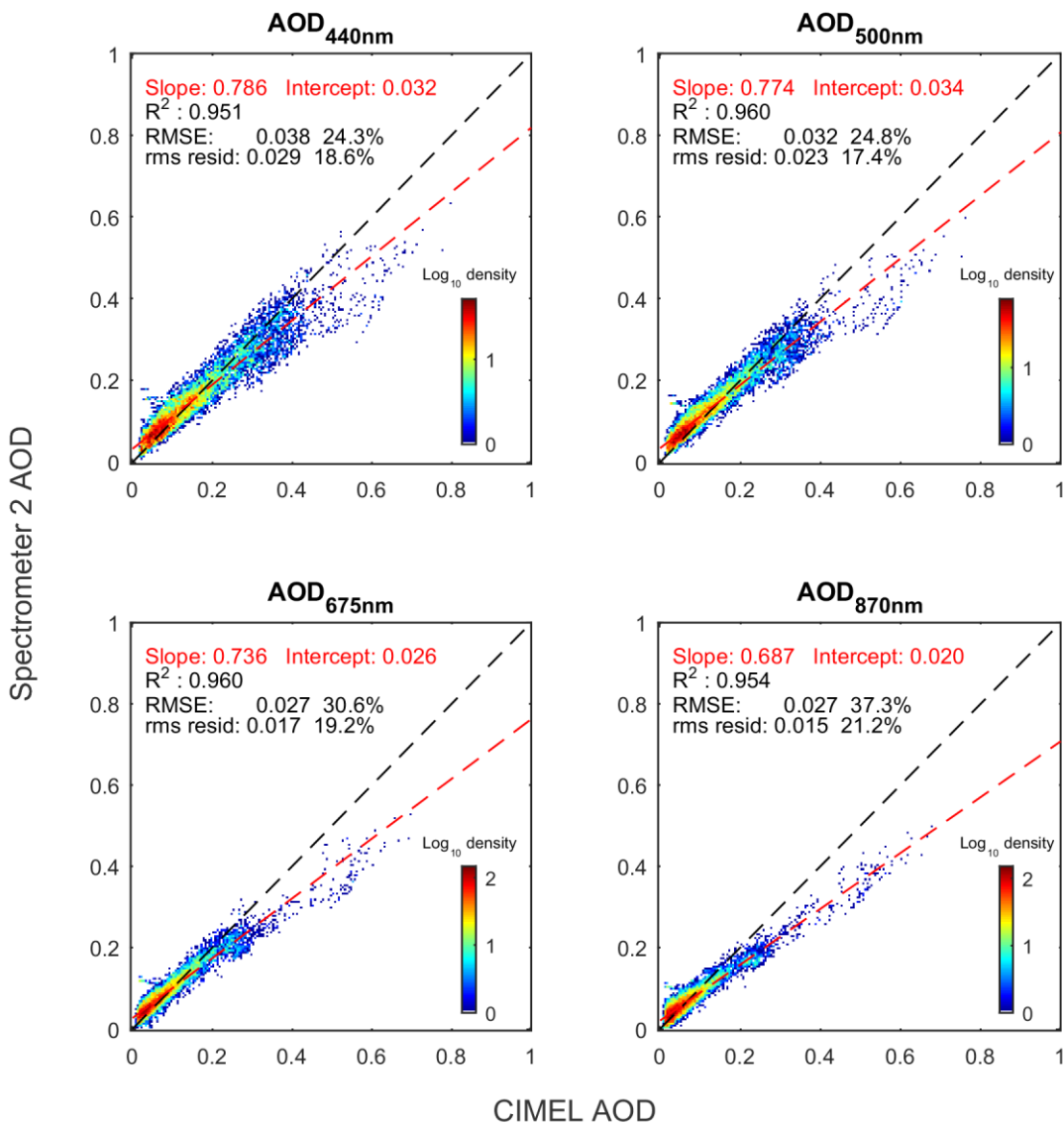
Figure 7: Spectrometer 2 (Zeiss) AOD results compared with CIMEL sun photometer at Burjassot, January 2015 – July 2016. These are log density plots: red points represent around 100 data points, whereas the blue points only a single data point. No further corrections applied.
