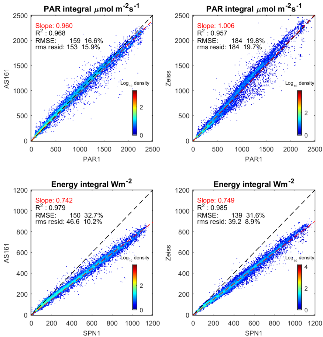
Figure 12: Comparisons of integrated PAR (400nm – 700nm, quantum weighting) and Energy (integrated over 380nm – 1050nm) with the adjacent Kipp & Zonen PQS-1 PAR sensor, and SPN1.
