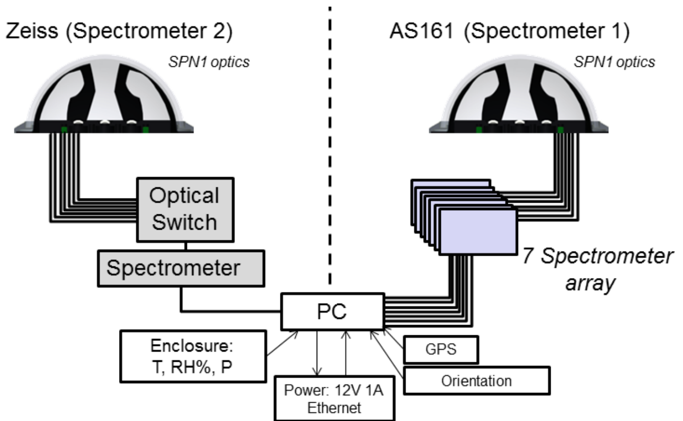
Figure 2: System diagram for the two spectrometer configurations. Elements in white are common to both configurations, although each have their own separate PC, GPS etc. Main configurational difference is that the AS161 (Spectrometer 1) contains seven spectrometers, whereas the Zeiss (Spectrometer 2) contains only one which is connected to the seven optical channels via an optical switch. The PC enclosure temperature (T), relative humidity (RH) as well as atmospheric pressure (P) is monitored.
