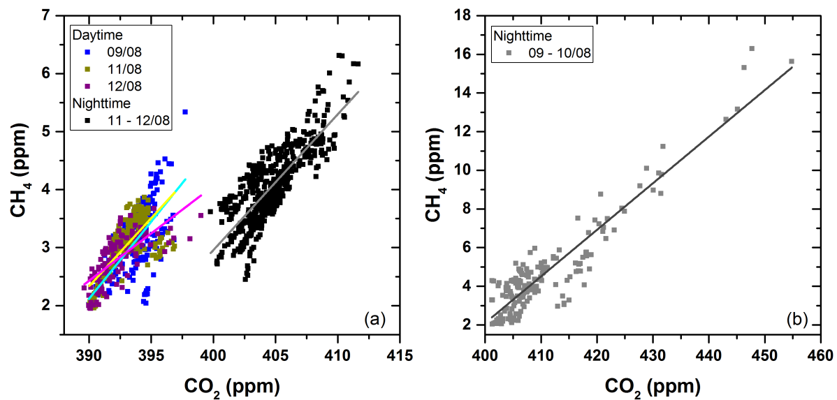
Figure 3. Determination of the enhancement factor as the linear regression slope of \chi_{\text{CH}_4} versus \chi_{\text{CO}_2} separately for three days (09:00 to 18:00 UTC) and two nights (21:00 to 06:00 UTC) influenced by air from the active site. Data are shown in two separate panels to account for the different scales.
