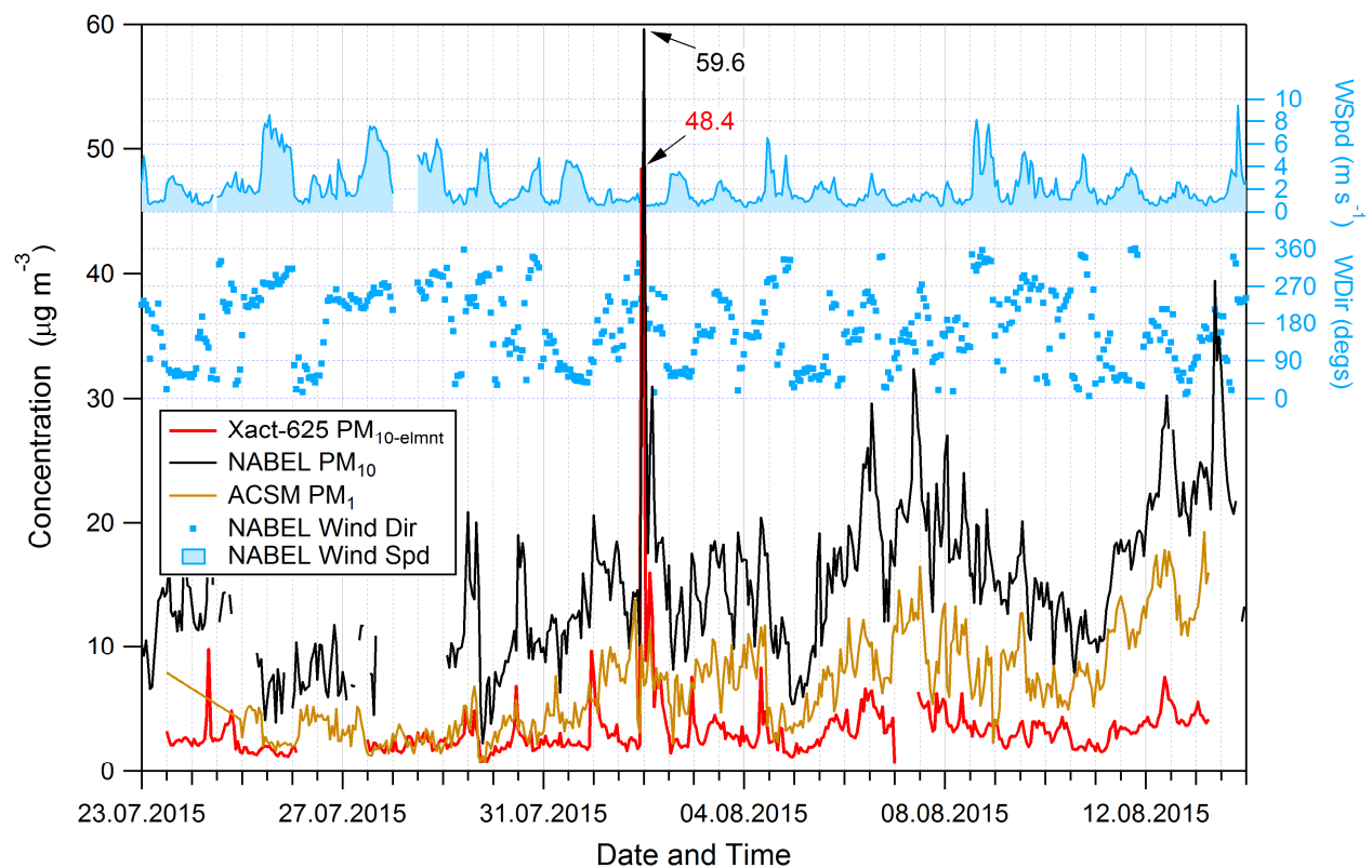
Figure 4: Time series of Xact625 total elemental concentration, ACSM PM1 data, NABEL TEOM \text{PM}_{10} data, and wind speed (WSpd) and direction (WDir) measurements in Härkingen. Numbers at the peaks indicate 1-h concentration maxima.
