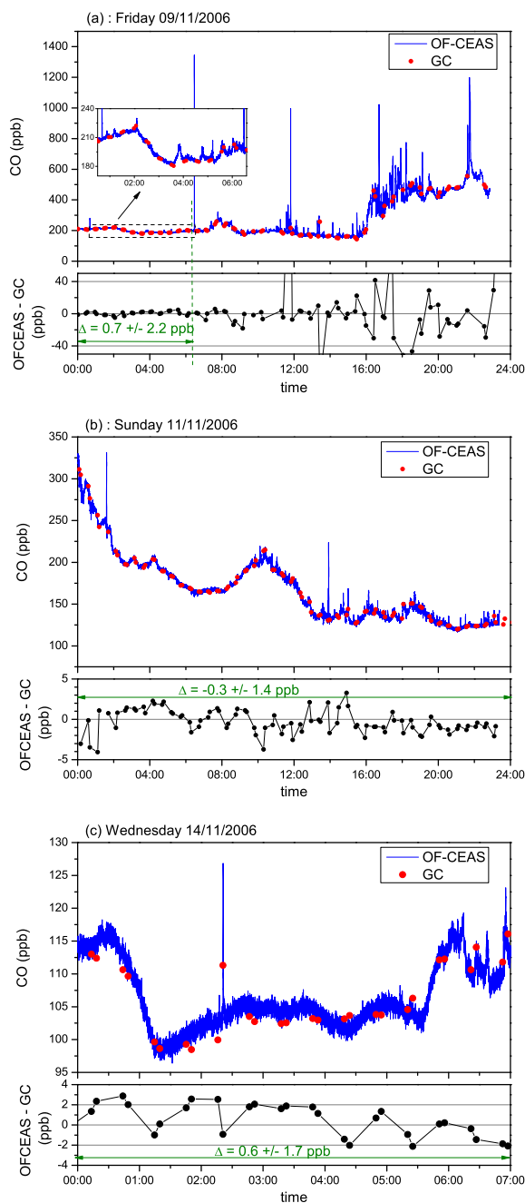
Figure 2. Two days and one night monitoring of atmospheric concentration in Gif sur Yvette selected for their different ranges. CO values are given in dry air mole fraction. The GC data are time-shifted by 14 min in order to eliminate time delay between the two instruments. Upper graphs: OF-CEAS measurements are averaged for 2 s while GC measurements are performed twice an hour. Lower graphs: Difference of the measurements after averaging OF-CEAS data for 1 minute around the GC time measurement. Mean values of the difference and standard deviations are written in green.
