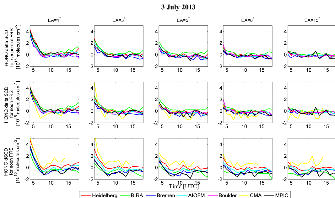
Figure 3: Time series of the hourly averaged values of HONO delta SCDs using a sequential FRS and a daily noon FRS as well as the HONO dSCDs with a daily noon FRS for different elevation angles and participating instruments on 3 July 2013.
