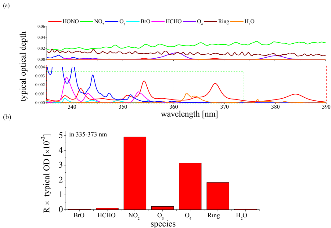
Figure 11: (a) Typical optical depths of the absorption species as the function of wavelength in the wavelength range for HONO retrieval; the dashed colored squares in the lower subplot indicate the wavelength ranges 335 nm up to 360 nm, 373 nm and 390 nm, respectively; (b) Correlation coefficients of the different cross sections multiplied with typical optical depths of respective species (based on the measurements during the whole campaign) with the HONO cross sections in the spectral range 335-373 nm.
