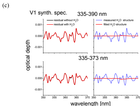
Figure 10: (a) Residual structures (left) and H 2 O fit results (right) for the same measured spectrum as in Fig. 9 for the fits either with (red) or without (black) the POKAZATEL H 2 O cross section. The upper and lower two subfigures represent fits in the spectral range of 335-390 nm and 335-373 nm, respectively. (b) and (c) are same as (a), but for the V2 and V1 synthetic spectra for a SAA of 166° and EA of 1°, respectively.
