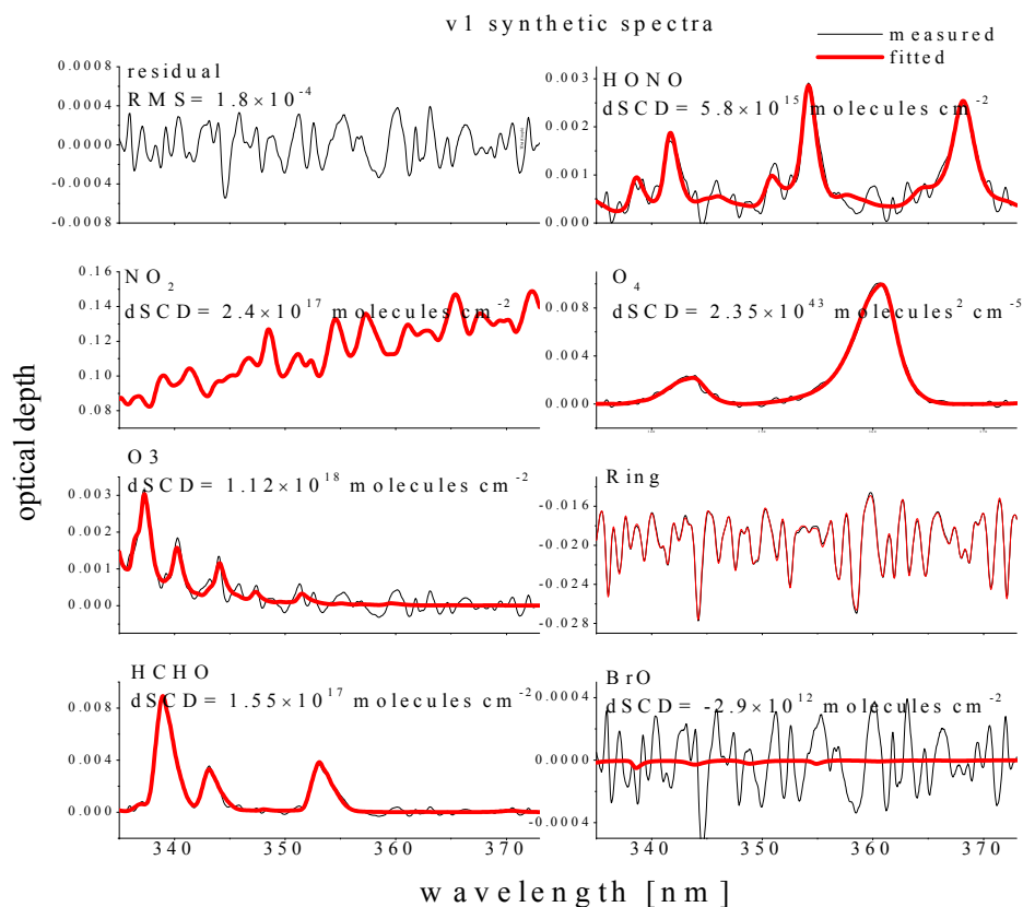
Figure 7: Example of a HONO fit of a V1 synthetic spectrum for a SAA of 166^\circ and EA of 1^\circ using the DOAS setting with a sequential FRS without the intensity offset correction (setting #4 in Table 4).
