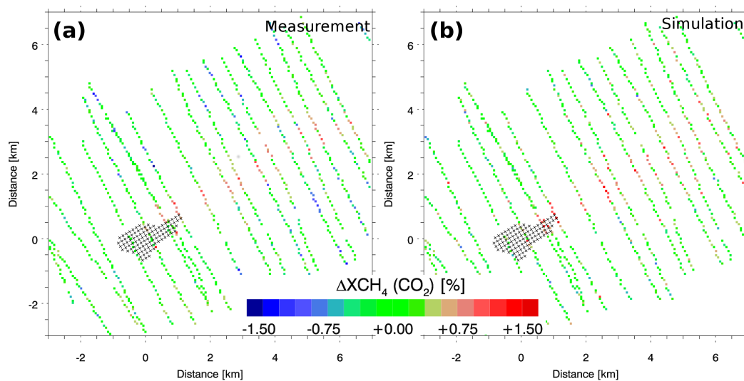
Figure 12. Shown are CH_4 variations relative to the background column for the Olinda Alpha Landfill in the 01.09.2014. (a) Shows the actual acquired data set similar to that show in Fig. 1 and (b) shows the results from the OSSE. Both data sets are gridded. The crosses represent the sources which were used in the OSSE and are homogeneously distributed across the landfill. The wind direction was south-west. For further details see text and supplementary material Sect. S8.
