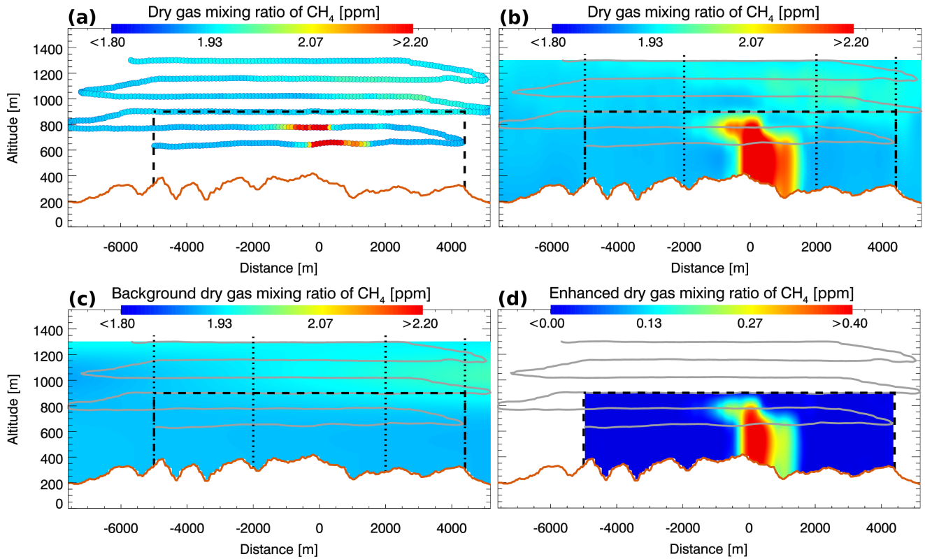
Figure 5. Example dry gas mixing ratios of CH 4 for the first downwind wall measured on the 01.09.2014 (middle in-situ wall in Fig. 6, solid red line). (a) Projected and time lag corrected mixing ratios acquired along the flight track onto the wall. (b) Kriged mixing ratios based on the measurements in (a) and an additionally added pseudo-track at the surface (not shown, see Sect. 4.2 for details). (c) Derived background mixing ratios from (b). (d) Derived CH 4 enhancement (kriged mixing ratios in (b) minus background mixing ratios in (c)). X-axis gives the distance from the approximate plume centre in m and y-axis gives the altitude in m above sea level (m asl). Solid orange lines depict the surface elevation (based on SRTM) and solid grey lines the projected flight track. Vertical dotted black lines show horizontal limits, which were used to define the background area (here: from -5.0 to -2.0 km and from +2.0 to +4.4 km). The area, which was used in the mass balance approach for estimating the emission rate, is enclosed by the dashed black lines.
