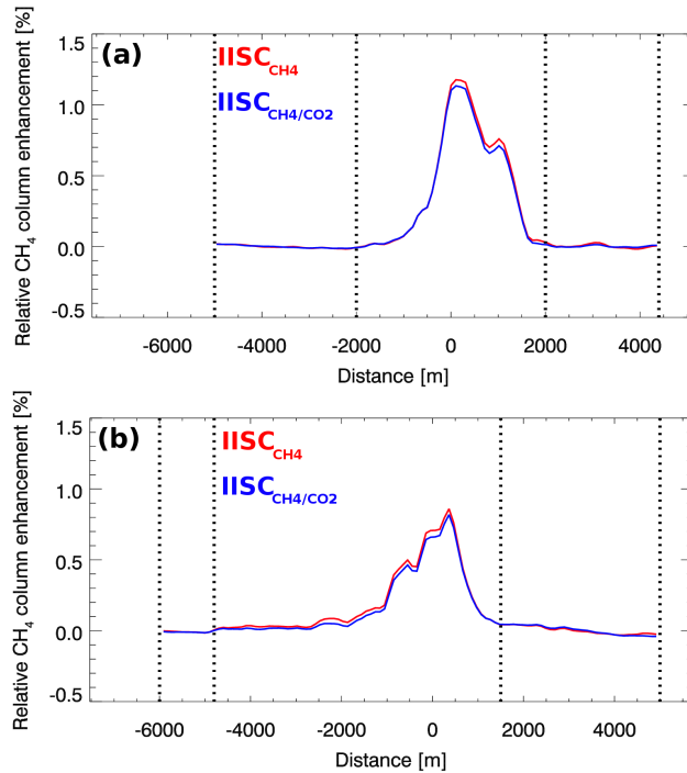
Figure 8. Cross-sections of the relative CH 4 column enhancements determined from the integrated in-situ columns (IISCs) as discussed in Sect. 3.1.1 of the first (a) and second (b) downwind wall of the Olinda Alpha Landfill measurements on 01.09.2014. The blue solid lines (IISC CH 4 /CO 2 ) represent the cases which are influenced by the co-emitted CO 2 , whereas the red solid lines (IISC CH 4 ) are not. The measurements enclosed by the black dotted lines and located at the flanks / edges of the plume are used for normalization and determination of the background.
