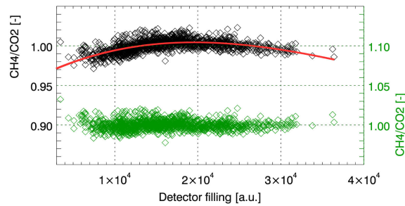
Figure 3. Scatter plot of the ratio of the retrieved CH 4 and CO 2 column over the maximum detector filling on the 01.09.2014. Black diamonds: Non-corrected data, left scale. Red solid line: Fitted 3 rd order polynomial. Green diamonds: Corrected data, right scale.
