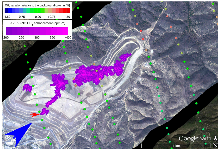
Figure 11. The MAMAP remote sensing (coloured circles) and the AVIRIS-NG (pink shaded areas) measurements on the 03.09.2014 are shown. The RGB map underneath is also based on AVIRIS-NG observations. For better source attribution, only AVIRIS-NG measurements having a methane column enhancement of larger than 200 ppm · m are shown. The non threshold filtered flight track is depicted in the Fig. 9 (b). The blue arrow depicts the approximate wind direction. Map underneath visible in the upper left and bottom right corner is provided by Google Earth.
