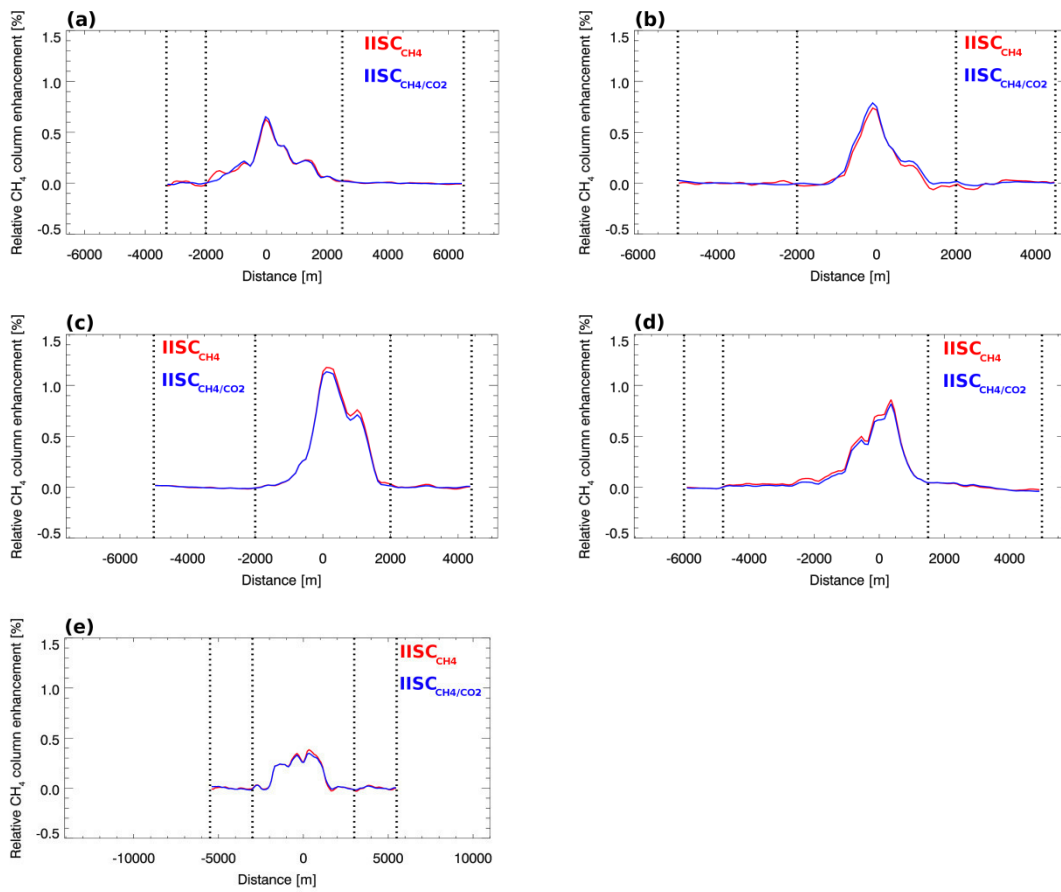
Figure S 17. As Fig. 7 but for all downwind walls. (a) 27.08.2014. (b) 28.08.2014. (c) 01.09.2014, first downwind wall (as in Fig. 7, a). (d) 03.09.2014, second downwind wall (as in Fig. 7, b). (e) 03.09.2014.
