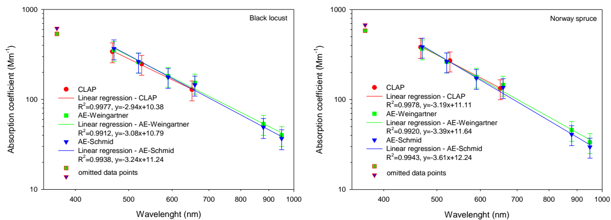
25 Figure 3. Absorption Ångström exponent of tar balls prepared from the liquid distillate of black locust and Norway 26 spruce. The linear equations are calculated for the log A vs. log \lambda values.
