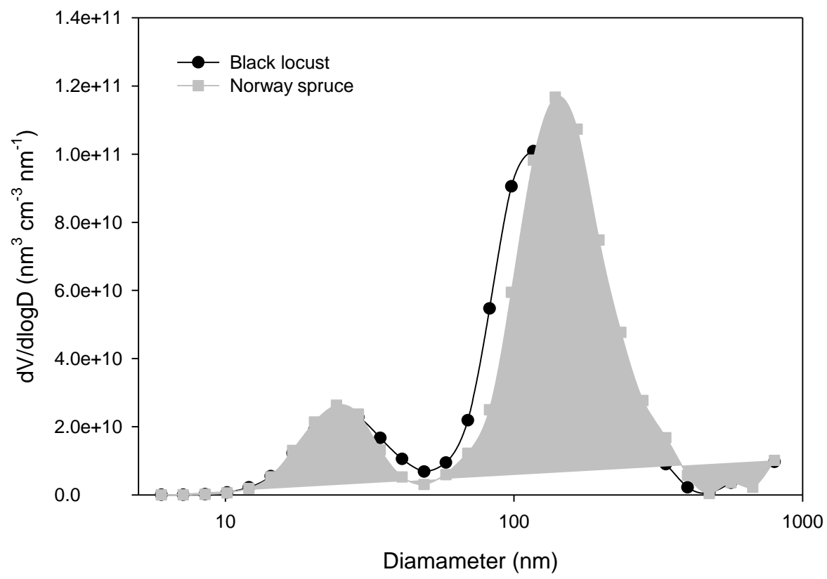
22 Figure 2. Examples for the measured size distribution of laboratory generated tar balls from the dry distillate of black 23 locust and Norway spruce.
