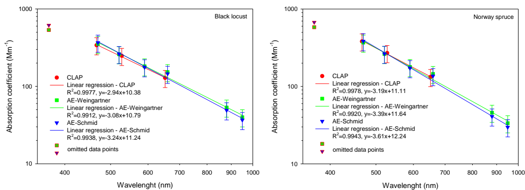
18 Figure 3. Absorption Ångström exponent of tar balls prepared from the liquid distillate of black locust and Norway 19 spruce. The linear equations are calculated for the log A vs. log \lambda values.
