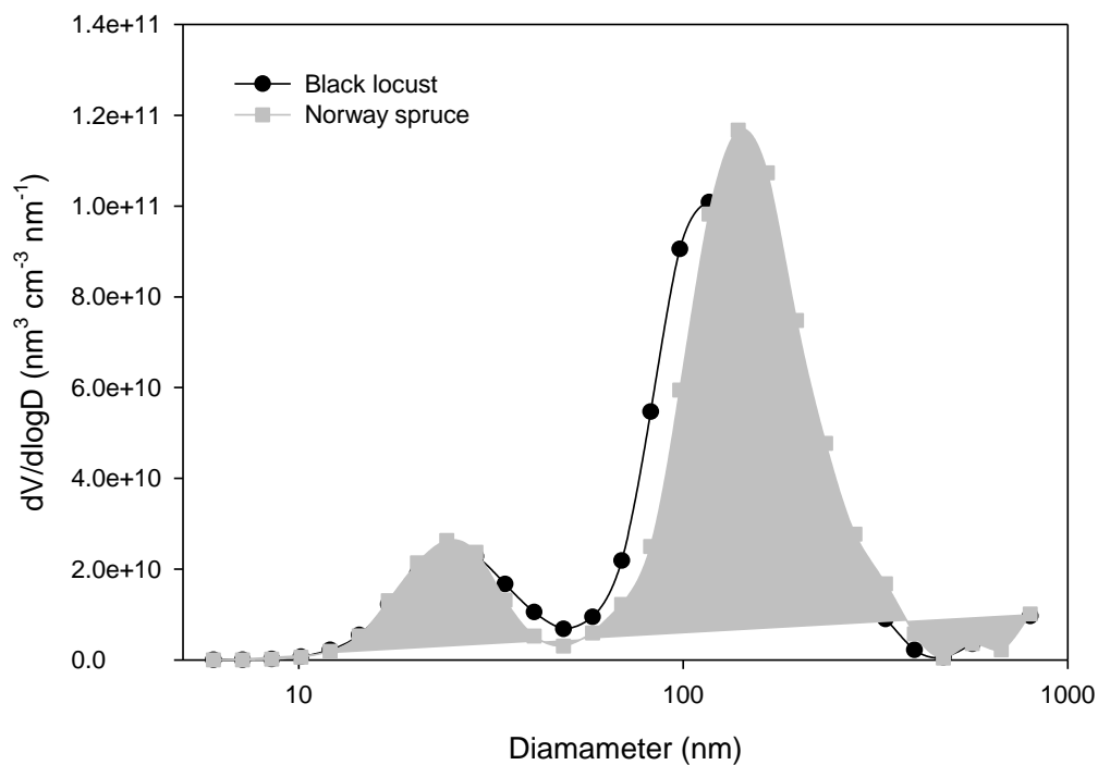
15 Figure 2. Examples for the measured size distribution of laboratory generated tar balls from the dry distillate of black 16 locust and Norway spruce.
