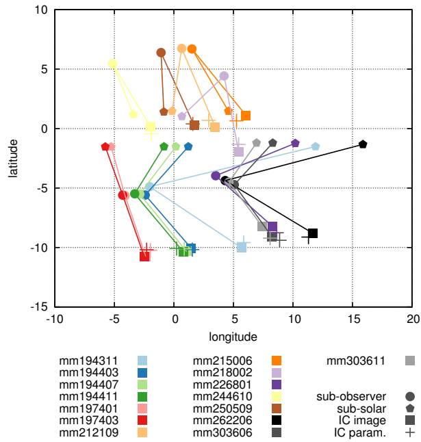
Figure 8. Illustration of the IC parametrisation. For each ROLO reference image, the sub-observer point P_{\text{sobs}} , the sub-solar point P_{\text{ssol}} and the IC location in the ROLO images P_{\text{icen}} are plotted onto a grid of lunar coordinates. The parameterised IC (shown as cross) is in all cases close to the observed intensity centre.
