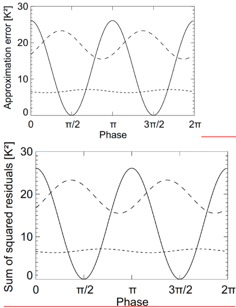
Figure 4: Dependence of the sum of squared residuals approximation error on the phase of the wave with a wavelength of 3.0 km and a distance of 1.4 km (short dashes), 1.5 km (solid line) and 1.6 km (long dashes) between two spline sampling points.
