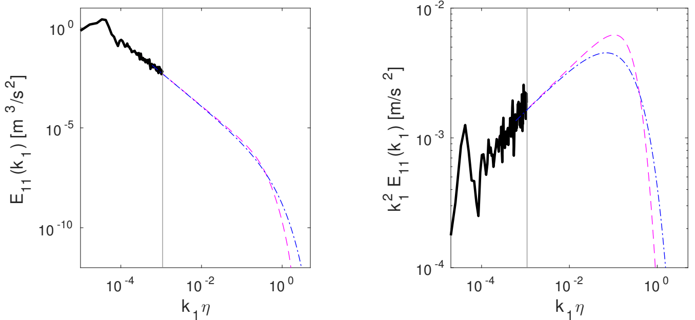
Figure 12. One-dimensional spectra: black solid line - measured part, dashed magenta line - recovered part with f_\eta described by Eq. (23), dot-dashed blue line - recovered part with f_\eta described by Eq. (24), a) energy spectrum E_{11}(k_1) , b) k_1^2 E_{11}(k_1) .
