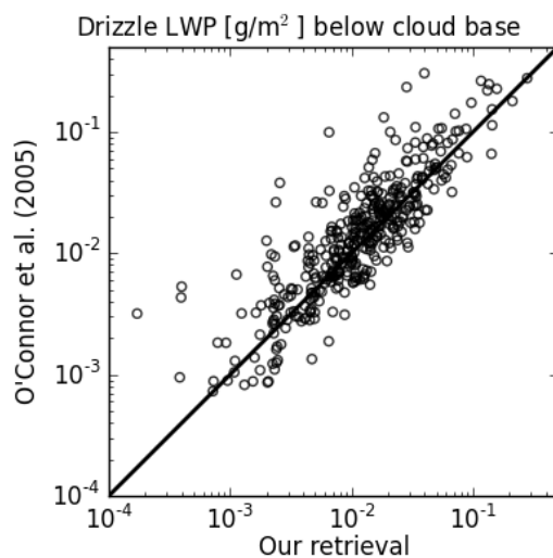
Figure 12. Comparison with the drizzle liquid water path below the cloud base as retrieved using the technique of O'Connor et al. (2005), available as one of the Cloudnet products. The diagonal line marks the one-to-one correspondence.
