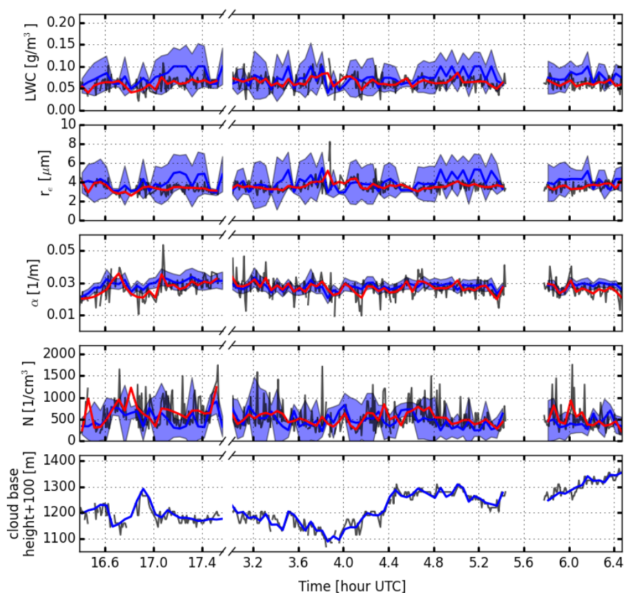
Figure 9. Time series of the optical and microphysical properties of the cloud at 100 m above the cloud base. The break along the horizontal axis marks the change of day from Oct 25 to Oct 26. The data around 5.6 hr is deemed unsuitable for retrieval using the depolarization lidar method. The cloud properties and their respective uncertainties derived using the depolarization method are shown by the blue lines and the shaded area. The results of our retrieval are represented by the black lines (temporal resolution: 30 sec) and red lines (time average, to match the time stamps and the 180-sec resolution of the depolarization results). Top to bottom: liquid water content, effective radius, extinction coefficient, number concentration and the altitude at which the cloud properties are evaluated.
