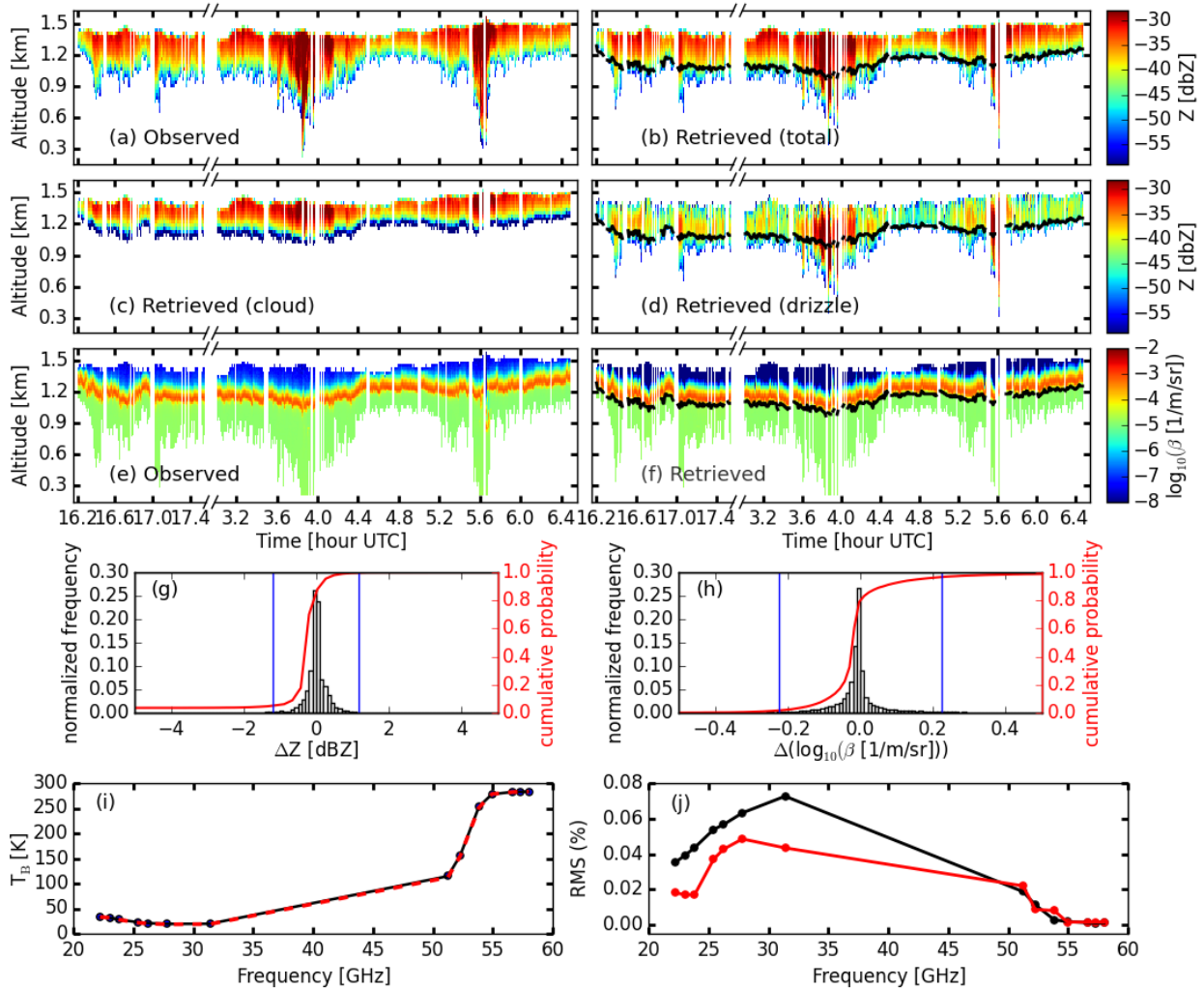
Figure 6. Measured and retrieved signals of the selected cases from the ACCEPT campaign. The breaks along the horizontal axes in (a)-(f) mark the change of date from October 25 to 26, 2014. Panels (a)-(d) show the radar reflectivity as observed and as retrieved, along with the decomposition into drizzle and cloud reflectivities. The black line delineates the cloud base determined in the retrieval. Panels (e)-(f) display the observed and the retrieved attenuated lidar backscatter \beta . Panels (g) and (h): histograms of the differences between the observed and the retrieved (total) signals (observed - retrieved). The red curves show the cumulative distributions. The spread of the distribution is indicated by the blue vertical lines that mark the interval within which 95% of the total occurrences are found. Panel (i) shows the brightness temperatures T_B averaged over distance at each frequency channel: black circles and line show the observations while the dashed red line shows the retrieval. In (j) we plot the standard deviation of the observation mean divided by the mean itself (black) and the RMSD between the retrieval and the observation, divided by the observation mean (red).
