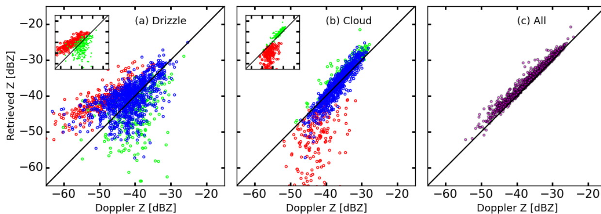
Figure 10. Radar reflectivity from our retrieval ('retrieved Z') plotted against those derived from the Doppler spectral decomposition ('doppler Z'). Drizzle, cloud and total reflectivities are shown separately in (a), (b), (c), respectively. The points are color-coded according to their location in the cloud. Red points are from the cloud base area, blue points from the middle of the cloud and green points are from the cloud top region (see the text for details). The insets in (a) and (b) show the same plot with the blue points excluded. The diagonal line is the one-to-one line.
