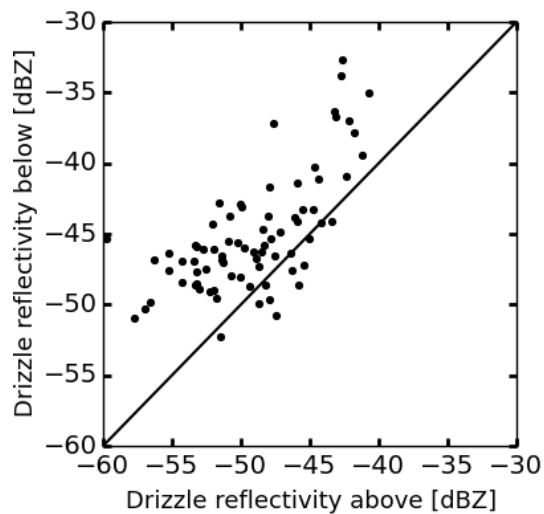
Figure 11. Comparison between the drizzle reflectivities at one range gate above and one range gate below the cloud base. The reflectivities above the cloud base are obtained from the Doppler spectral decomposition. The ones below the cloud base are simply the observed reflectivity. The diagonal line marks the one-to-one correspondence.
