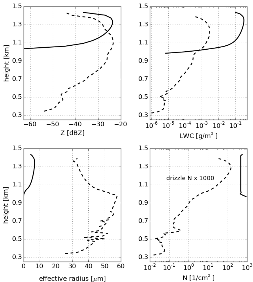
Figure 8. Mean vertical profiles of the cloud (solid lines) and drizzle (dashed lines) properties from the observation on October 26, 2014 between 3.8 and 4.0 hr UTC. Clockwise from the top left: radar reflectivity factor in dBZ, liquid water content in g/m 3 , number density per cm 3 and effective radius in microns. Note that the number density of the drizzle has been multiplied by a factor of 1000 for illustration purposes.
