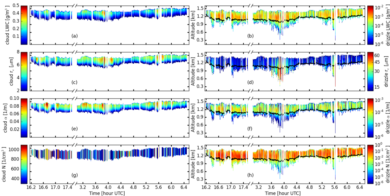
Figure 7. Optical and microphysical parameters of the cloud (left) and the drizzle (right) as obtained from the retrieval, as a function of time and height. From top to bottom: liquid water content, effective radius, extinction coefficient and number concentration.
