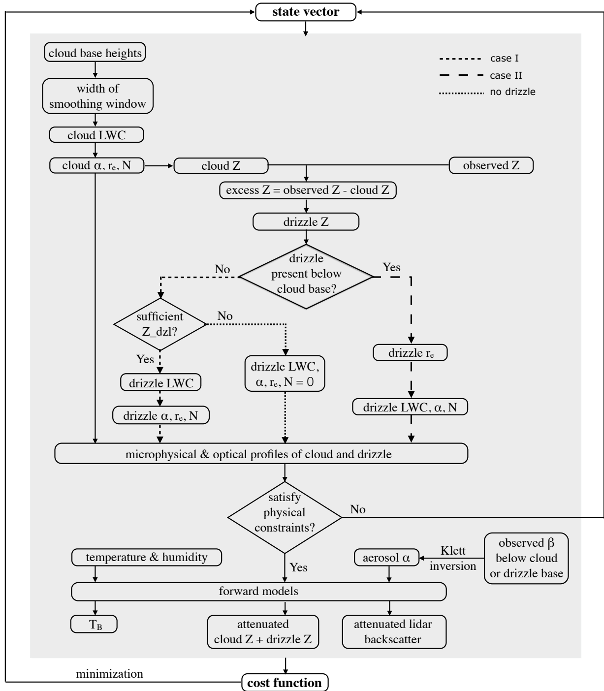
Figure 1. The retrieval flow-chart
