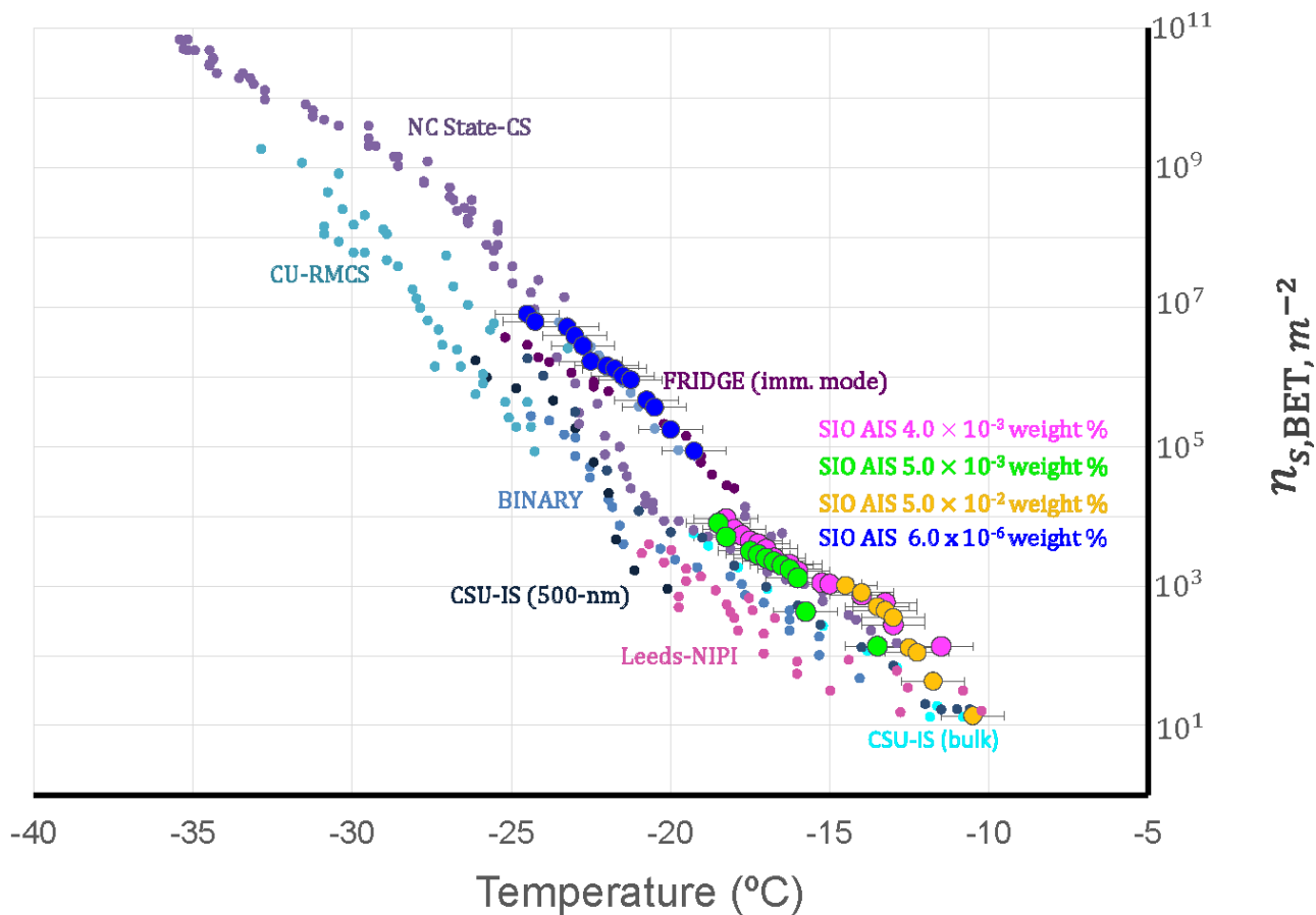
5 Figure 9: Immersion freezing spectra of illite NX particles in terms of n_{s,BET}(T) for comparison of SIO AIS against six other immersion mode techniques reported (see Hiranuma et al., 2015). n_{s,BET} is used to estimate ice nucleation surface-site density from an N_2 adsorption-based specific surface area (Hiranuma et al., 2015). CSU-IS (500 nm) represents measurements made on illite NX particles that were mobility diameter size-selected, whereas all other measurements reported were of bulk illite NX samples. Four different dilutions of illite NX suspensions were measured by the SIO AIS: 4.0 \times 10^{-3} wt %, 5.0 \times 10^{-3} wt %, 5.0 \times 10^{-2} wt %, and 6.0 \times 10^{-6} wt%. SIO AIS measurements fall on the warm side of the spectra.
