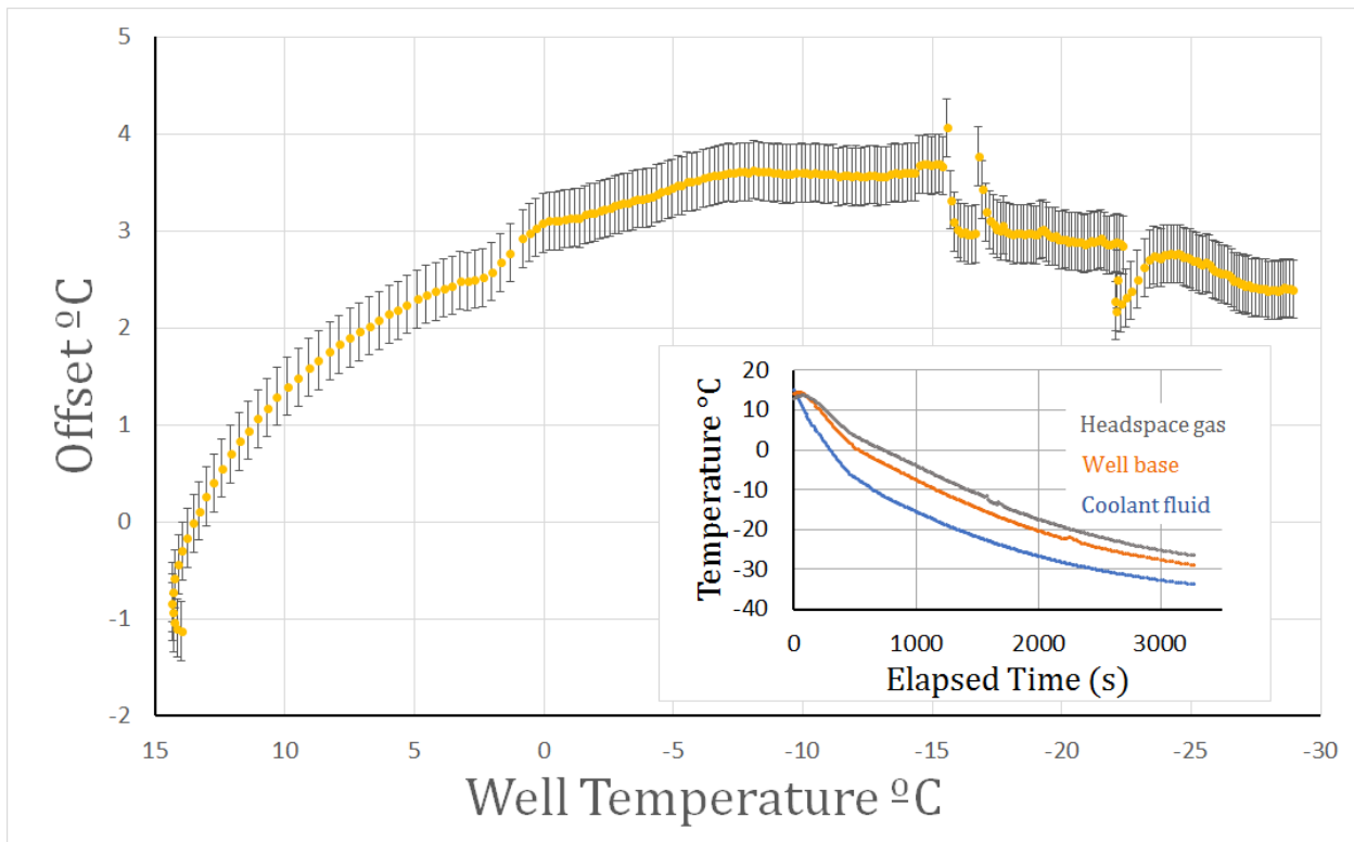
Figure 3: Graph of well temperature vs. temperature offset measured between the base of the well and the air above the well as measured with a thermistor probe (orange filled circles). The error bars in the larger plot show the range of temperature offsets corresponding to the \pm 0.3 °C calibration error of the temperature standard. From room temperature to -33 °C as measured at the base of the well, the average cooling rate is -0.87 °C \text{min}^{-1} . Inset shows cooling performance of the bath coolant, and the temperature within the well and gas above well over 3276s measured by thermistor probes. The average cooling rate at the base of the well during the time period from 0 °C to -27 °C, however is -0.69 °C \text{min}^{-1} because the cooling rate slows as the refrigerated cooling bath approaches its minimum temperature.
