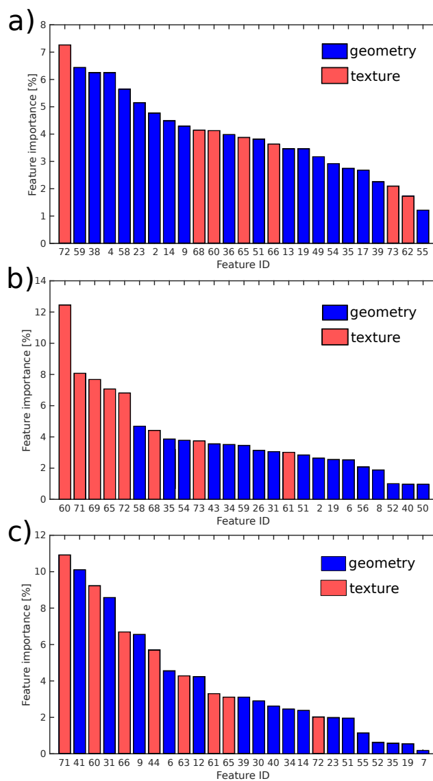
Figure 7. Estimation of the importance of each selected feature according to the logistic weights \beta_d for (a) hydrometeor type classification, (b) riming degree estimation and (c) melting snow detection. Descriptors computed only from the binary mask of the particle are displayed in blue (geometry) and descriptors using the textural information are in red (texture). Features ID are referring to Table A1.
