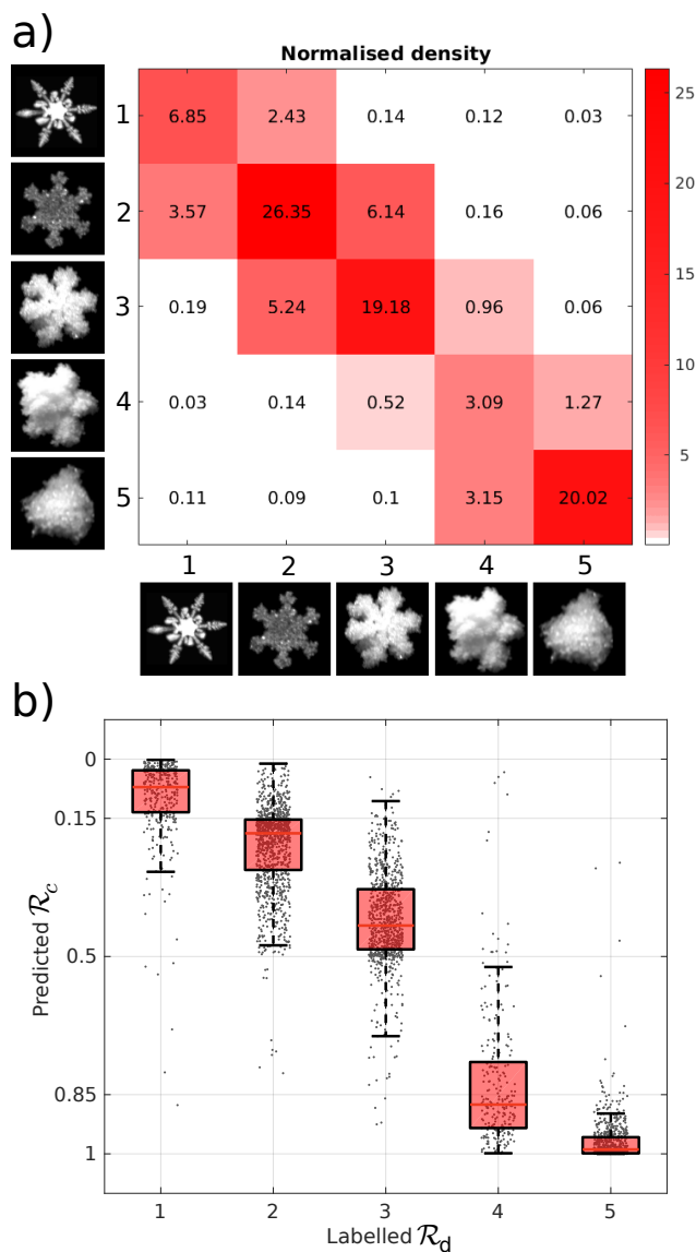
Figure 9. Illustration of the riming classification performance. (a) Confusion matrix of test data obtained by averaging 10 instances of 4-fold cross-validation. Labelled riming degrees are on the horizontal axis and predicted riming degrees \mathcal{R}_d on the vertical axis. (b) Boxplots of predicted riming index \mathcal{R}_c as a function of the labelled riming degree \mathcal{R}_d . The gray dots are the test data samples, horizontally spread around each value of \mathcal{R}_d to increase readability. The red lines are the medians, the boxes correspond to the interquartile range and the whiskers extend to 1.5x the interquartile range.
