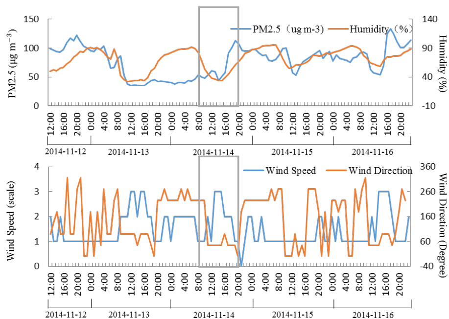
Fig. 3. Surface PM2.5 concentrations, relative humidity, wind speed and wind direction measured by Lin'an regional background station ( 30^{\circ}18' \text{ N} , 119^{\circ}44' \text{ E} ) on 12th-16th November
