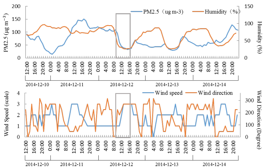
Fig. 4. Surface PM2.5 concentration, relative humidity, wind speed and wind direction measured by Lin'an regional background station ( 30^{\circ}18' \text{ N} , 119^{\circ}44' \text{ E} ) on 10th -14th December
