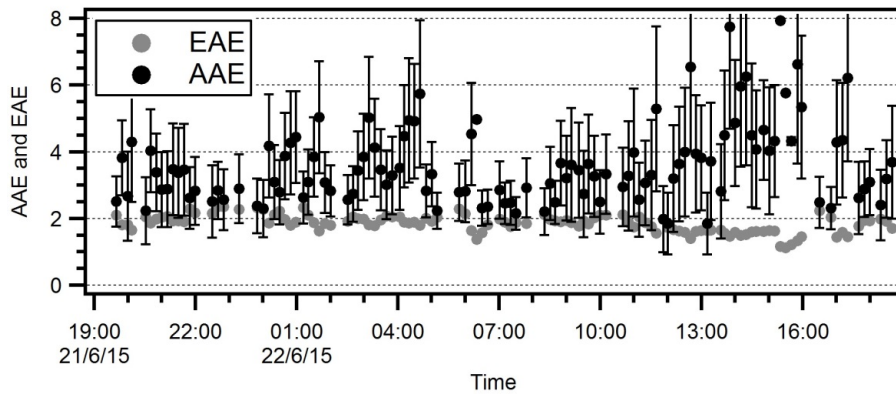
Fig. 1. Figure 9. Time series of the retrieved absorption and extinction Angstrom exponents (AAE and EAE) for the 300 to 650 nm wavelength range.
