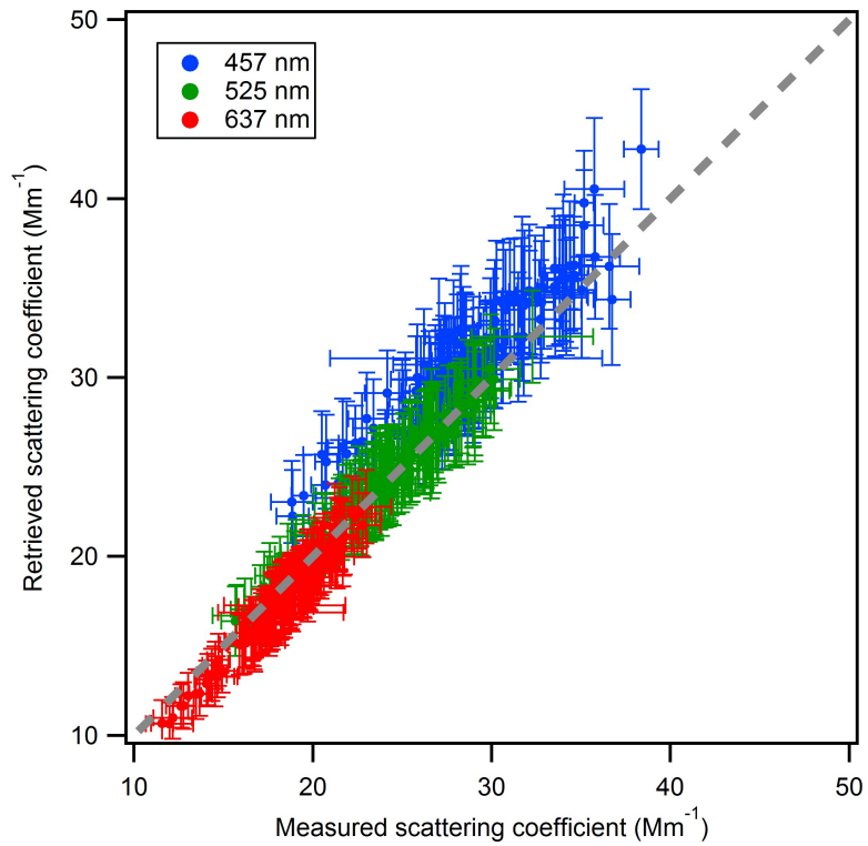
Fig. 2. Figure S3. Retrieved and measured scattering coefficients at the nephelometer wavelengths (457, 525 and 637 nm).
