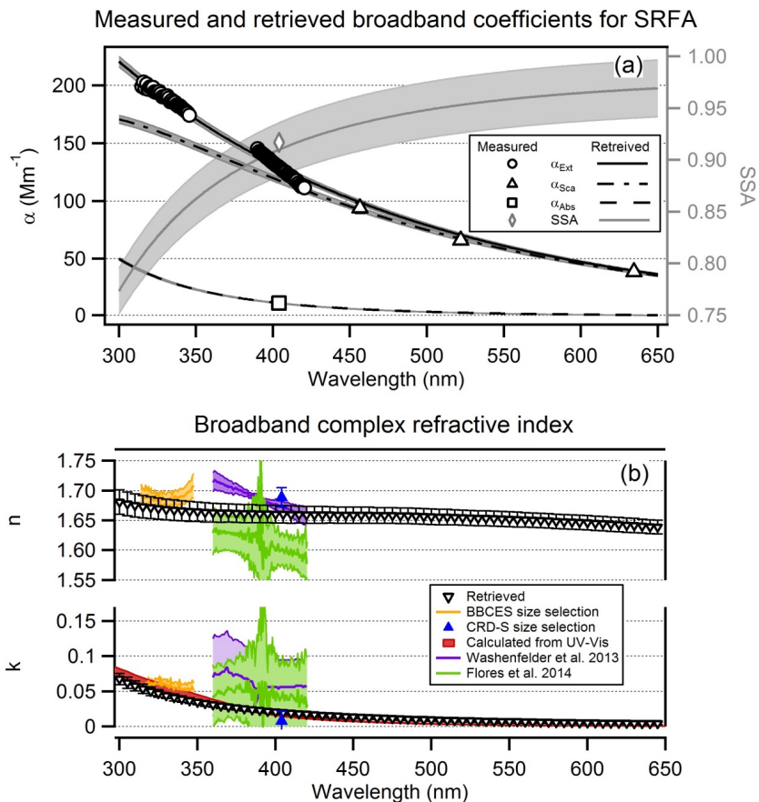
Fig. 2. Figure 6. (a) Measured extinction (circles), scattering (triangles) and absorption (square) coefficients ( \alpha_{\text{ext}} , \alpha_{\text{sca}} , and \alpha_{\text{abs}} , respectively) for Suwannee river fulvic acid (error bars representing me
