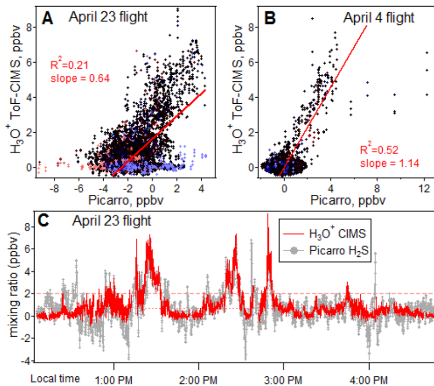
Figure 15. Scatterplot and time-series \text{H}_3\text{O}^+ comparison between \text{H}_3\text{O}^+ ToF-CIMS and Picarro CaRDS instruments. (a) Scatterplot of \text{H}_3\text{O}^+ ToF-CIMS vs Picarro \text{H}_2\text{S} for April 23 flight (Permian). Data points when the aircraft was ascending (red) and descending (blue) are highlighted. (b) Scatterplot of \text{H}_3\text{O}^+ ToF-CIMS vs Picarro \text{H}_2\text{S} for April 4 flight (Haynesville). (c) Time series during the April 23 flight. The \text{H}_3\text{O}^+ ToF-CIMS measurement has been averaged to a 6 second time basis. The Picarro \text{H}_2\text{S} is offset by 2 ppb (the intercept in panel a). The 1-s and 6-s detection limits for the \text{H}_3\text{O}^+ ToF-CIMS are shown by dashed red lines.
