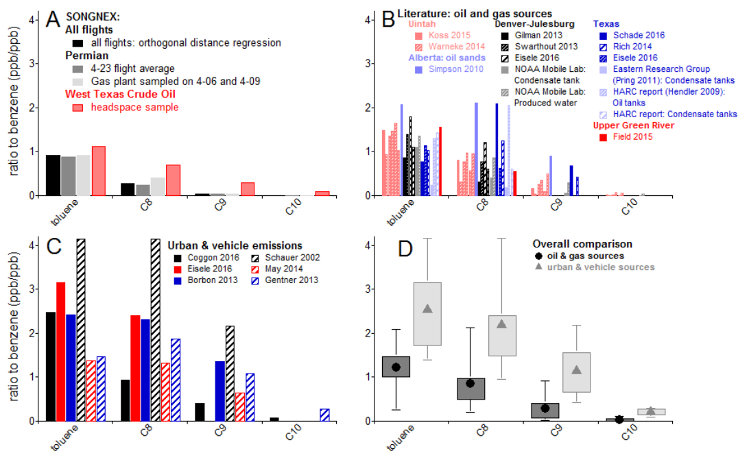
Figure 8. Comparison of C6-C10 aromatics distribution. Y-axis (molar ratio to benzene) is the same in each panel. (a) Measurements by H_3O^+ ToF-CIMS: SONGNEX flights and West Texas crude oil headspace. (b) Aromatic profiles from published studies of oil and gas fields, condensate tanks, oil tanks, and water storage tanks. (c) Aromatics profiles from published studies of urban areas and vehicle exhaust. (d) Average profiles of all oil and gas sources (panels a and b) and urban sources (panel c).
