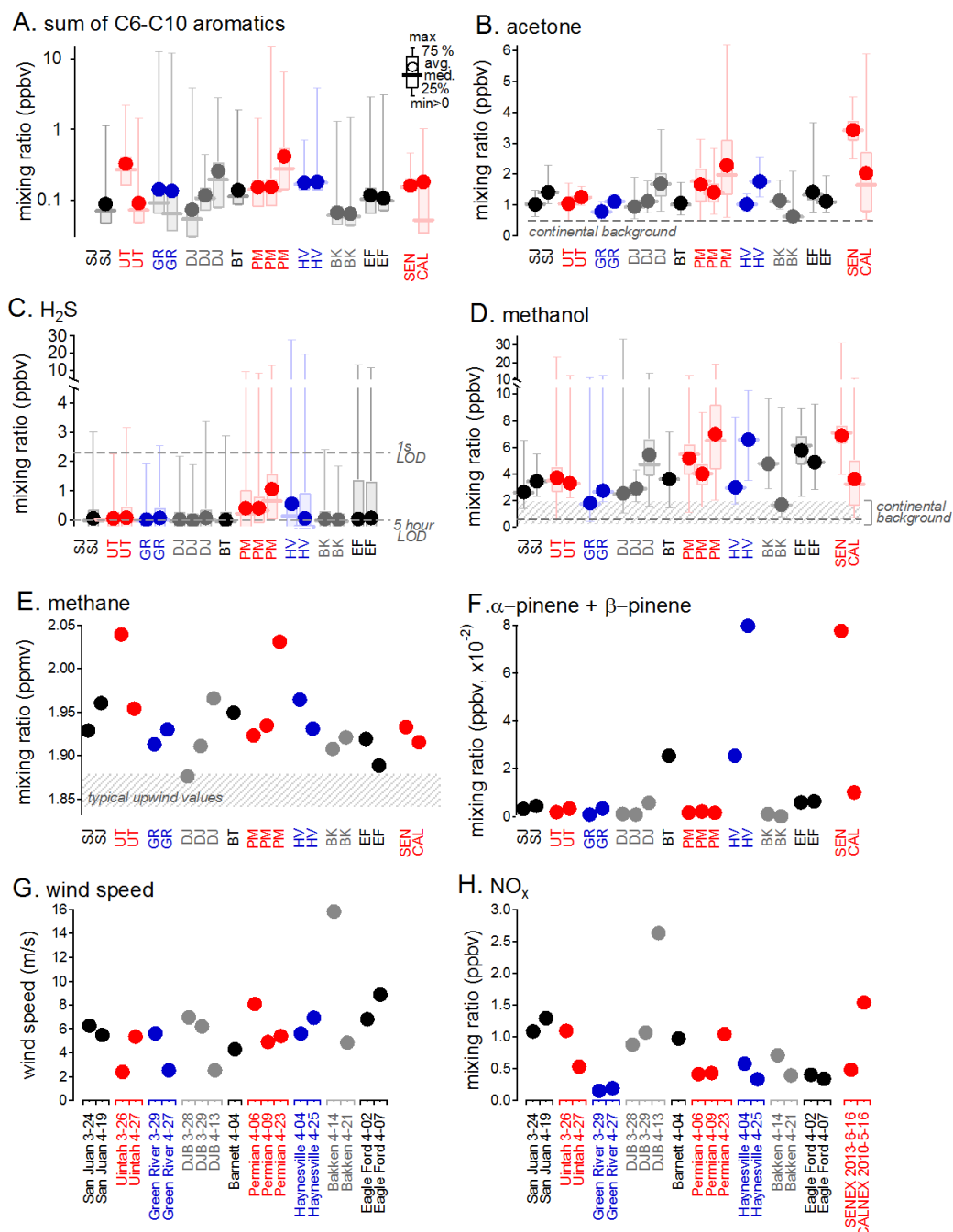
Figure 3. Mixing ratios observed within the boundary layer during SONGNEX flights. (a) Observed mixing ratios of aromatics (note log scale). (b) Mixing ratios of acetone. Tropospheric
