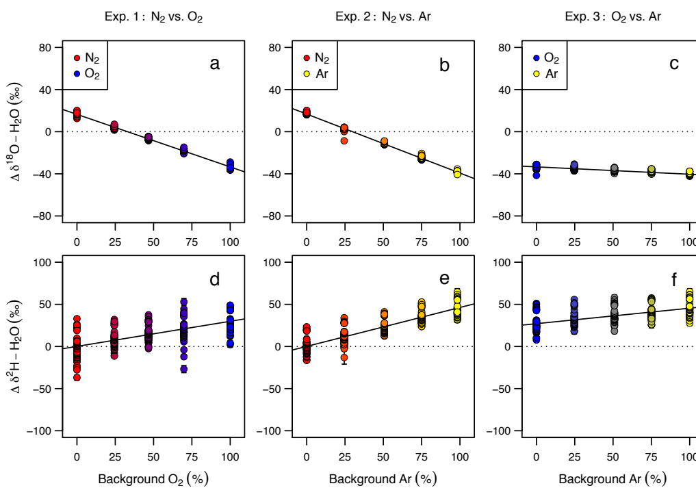
Figure 2. Sensitivity of \delta^{18}\text{O}-\text{H}_2\text{O} and \delta^2\text{H}-\text{H}_2\text{O} values to background \text{N}_2 , \text{O}_2 , and Ar mixing ratios. For each experiment, isotopic errors are plotted as the difference between the apparent and true isotopic composition of the standards (i.e., \Delta\delta^{18}\text{O}-\text{H}_2\text{O} = \delta^{18}\text{O}-\text{H}_2\text{O}_{\text{apparent}} - \delta^{18}\text{O}-\text{H}_2\text{O}_{\text{true}} and \Delta\delta^2\text{H}-\text{H}_2\text{O} = \delta^2\text{H}-\text{H}_2\text{O}_{\text{apparent}} - \delta^2\text{H}-\text{H}_2\text{O}_{\text{true}} ). For each panel, n = 330 measurements; points represent mean values \pm s.d.; and regression slopes are given by \beta_3 values in Table 2.
