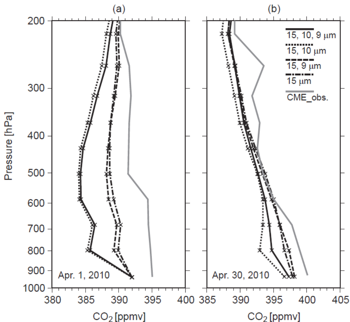
Figure 10. CO 2 profiles over Narita airport retrieved using four different wavelength bands of GOSAT/TANSO-FTS V161 5 LIB spectra: three bands, 15- \mu m, 10- \mu m, and 9- \mu m (thick lines); two bands, 15- \mu m and 10- \mu m (dotted lines); two bands, 15- \mu m and 9- \mu m (dashed lines), and the 15- \mu m band only (dashed-dotted lines). Nearby CME CO 2 profiles (CME_obs.) are shown by gray lines: (a) a case of April 1, 2010 and (b) a case of April 30, 2010.
