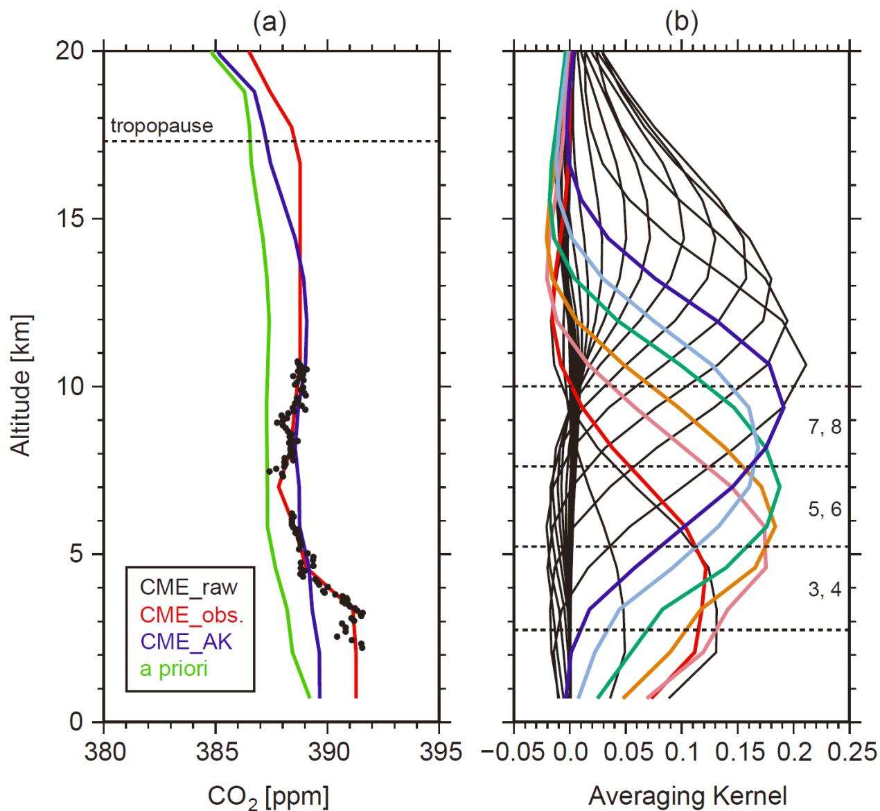
Figure 3. (a) Black circles represent original CME data (CME_raw), the red line shows an interpolated profile of the CME 5 data into GOSAT/TANSO-FTS TIR CO 2 28 retrieval grid layers (CME_obs), the blue line shows the interpolated profile to which TIR averaging kernel functions, shown in panel (b), are applied (CME_AK), and the green line shows a priori CO 2 profile.
