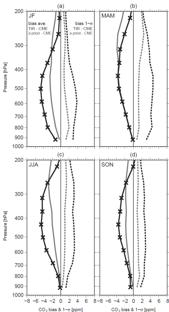
Figure 5. Bias profiles of GOSAT/TANSO-FTS TIR CO 2 data and a priori CO 2 data against CME_AK CO 2 data over Narita 5 airport and the 1- \sigma standard deviations for each retrieval layer and season in 2010. The CME_AK CO 2 data are CME CO 2 data to which TIR CO 2 averaging kernel functions are applied. Thick black and gray lines indicate the biases of TIR and a priori CO 2 data, respectively, and dotted black and gray lines show their 1- \sigma standard deviations. Cross symbols indicate the center pressure level of each retrieval layer: (a) JF, (b) MAM, (c) JJA, and (d) SON.
