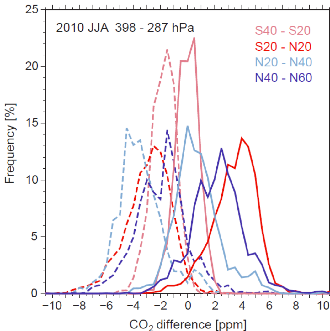
Figure 9. Same as Figure 7, but showing frequency distributions during the JJA season of 2010 on 398–287 hPa (retrieval 5 layers 7–8) for each latitude band. Pink, red, light blue, and blue lines shows the results from 40°S–20°S, 20°S–20°N, 20°N– 40°N, and 40°N–60°N, respectively.
