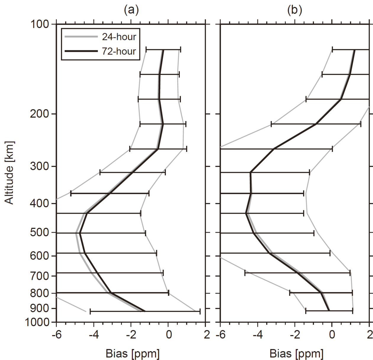
Figure 4. Bias profiles of GOSAT/TASNO-FTS TIR CO 2 data against CME_AK CO 2 data over Narita airport using coincident pairs with 24-hour (gray) and 72-hour (black) time difference criteria: (a) winter (JF) 2010 and (b) summer (JJA) 2010.
