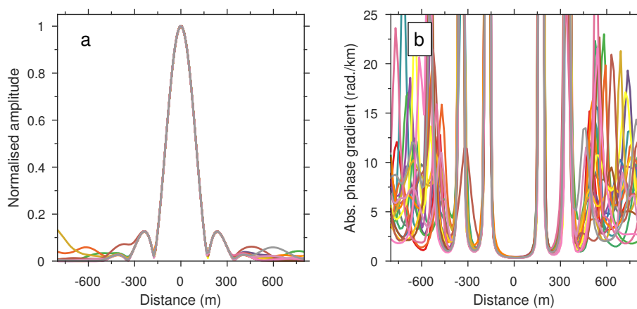
Figure 5. Impact of 20 wind turbines on weather radar I/Q data, recorded by radar Vara during September 2016. Panel (a) shows the average, normalised amplitudes of the wind turbine echoes while panel (b) shows the corresponding average, absolute phase gradient values.
