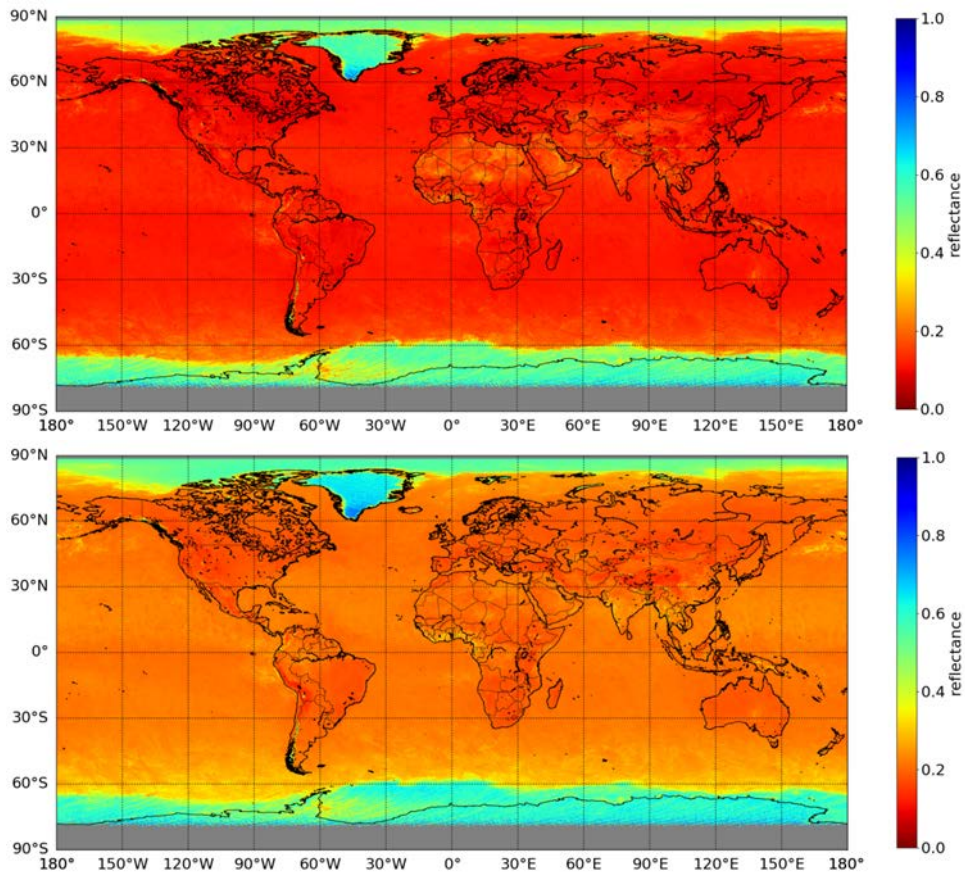
Figure 9: OCRA cloud-free background for G (top) and B (bottom) reflectances calculated using OMI data from August.
