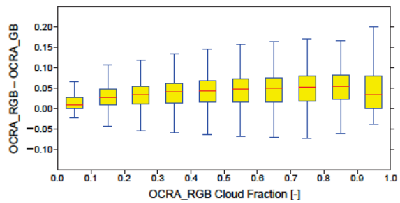
Figure 8: Box-and-whisker plot of the OCRA cloud fraction difference using RGB and GB colours retrieved using GOME-2 data from July 1 st 2012. The yellow boxes show the inter quartile range and median values are indicated as red lines. The overall median difference is 0.025.
