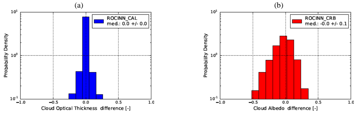
Figure 4: Histogram of the absolute differences between the simulated spectra and (a) the cloud optical thickness retrievals from ROCINN_CAL and (b) the cloud albedo retrievals from ROCINN_CRB. The retrieved cloud optical thickness varies from 2 to 50, with the cloud albedo ranging from 0 to 1.
