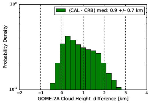
Figure 13: Histogram of the absolute differences between the GOME-2A cloud heights derived from ROCINN_CAL and ROCINN_CRB as seen in Figure 124.
