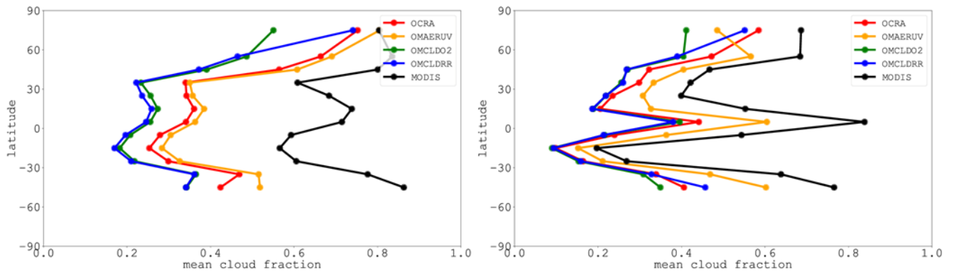
5 | Figure 11: Comparison of cloud fraction zonal means for results from the four OMI algorithms as seen in Figure 109 and from the MODIS measurements regridded to the corresponding OMI ground pixels. The left panel shows only measurements over ocean, while the right panel shows only measurements over land.
