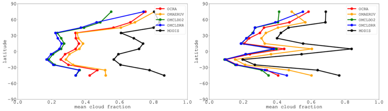
5 Figure 11: Comparison of cloud fraction zonal means for results from the four OMI algorithms as seen in Figure 10 and from the MODIS measurements regridded to the corresponding OMI ground pixels. The left panel shows only measurements over ocean, while the right panel shows only measurements over land.
