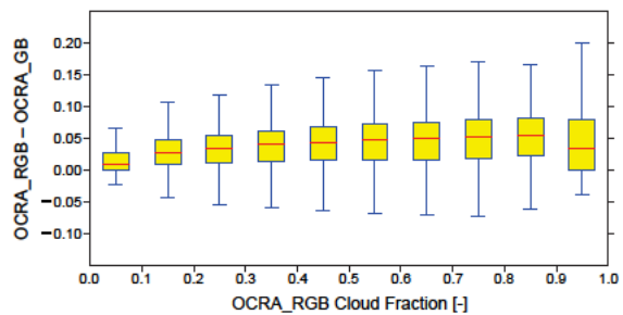
Figure 8: Box-and-whisker plot of the OCRA cloud fraction difference using RGB and GB colours retrieved using GOME-2 data from July 1 st 2012. The yellow boxes show the inter quartile range and median values are indicated as red lines. The overall median difference is 0.025.
