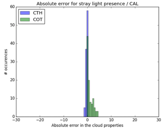
Figure 7: Absolute errors in the cloud properties due to the presence of stray light: (a) cloud height and cloud albedo errors for CRB and (b) cloud top height and cloud optical thickness errors for CAL.
