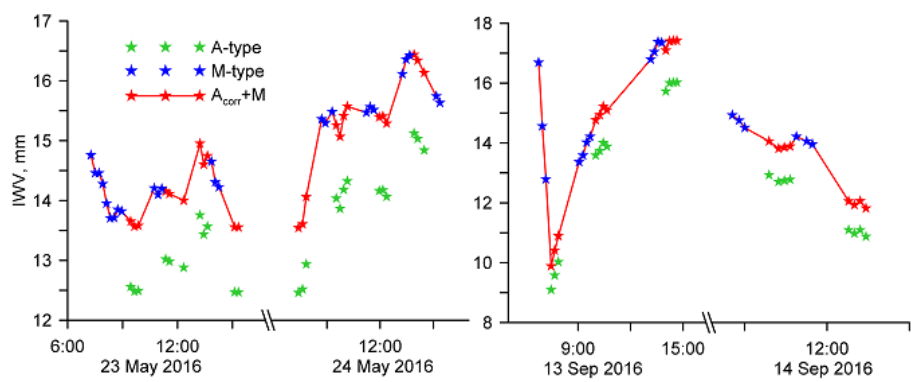
Figure 6. Diurnal variations of IWV content observed by FTIR technique: the A-type retrieval (green stars), the M-type retrieval (blue stars), and the joint A_{corr} and M-type retrieval (red line with stars).
