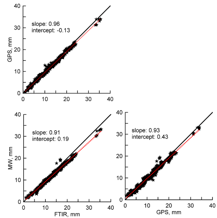
Figure 7. Correlation of IWV values measured by FTIR, GPS and MW techniques. Red dotted line is the linear regression line. The slope and intercept of linear regression line are given in each panel.
