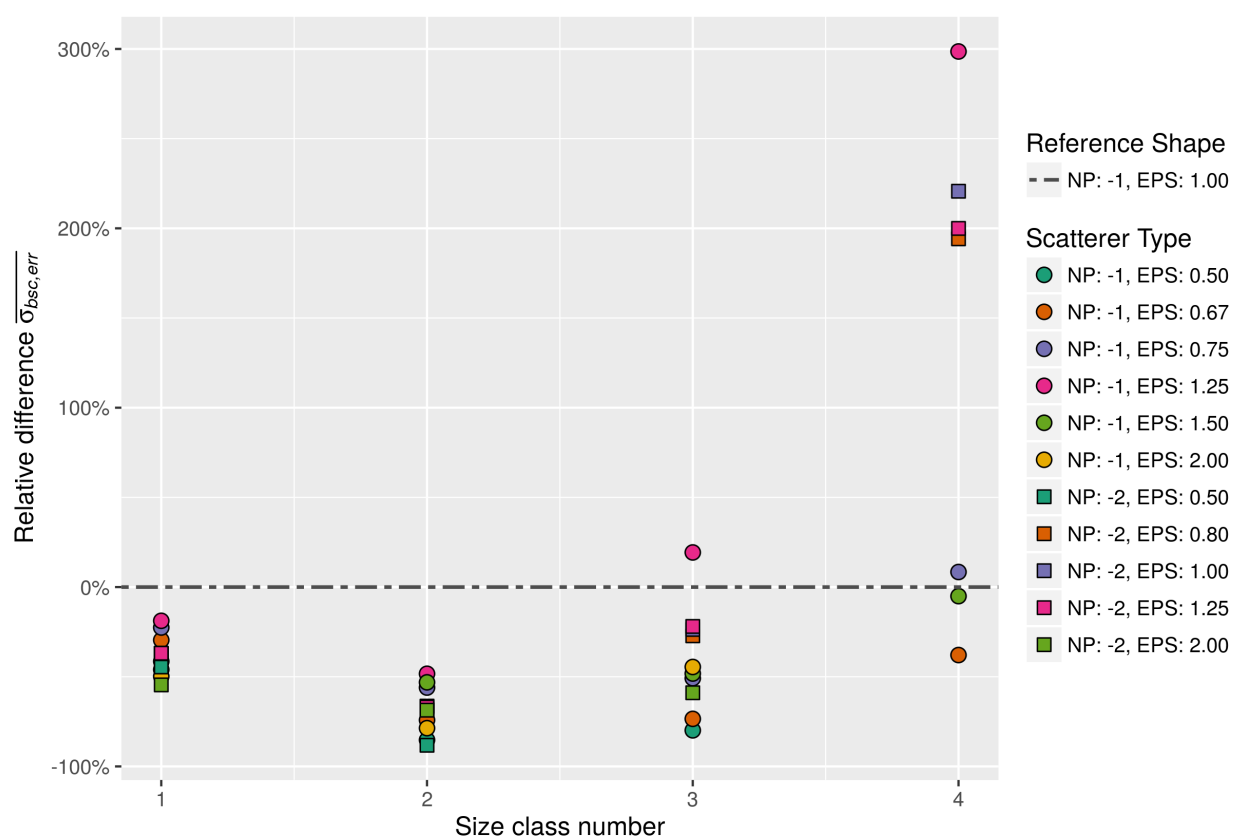
Figure 12. The same as Fig. 11 but for the effective backscatter cross section.
