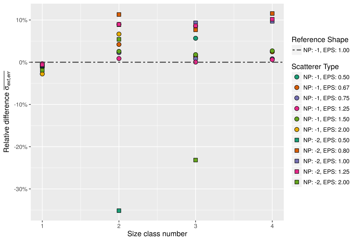
Figure 11. Relative errors of the effective extinction cross section if spherical particles are assumed but the real particles would be of elliptical (NP: -1) or cylindrical shape (NP: -2). Negative (positive) values indicate that spherical particles have larger (smaller) effective extinction cross section. Except for a strongly asymmetric cylinder, the effective extinction cross section of spherical particles are mostly smaller (up to 12 %).
