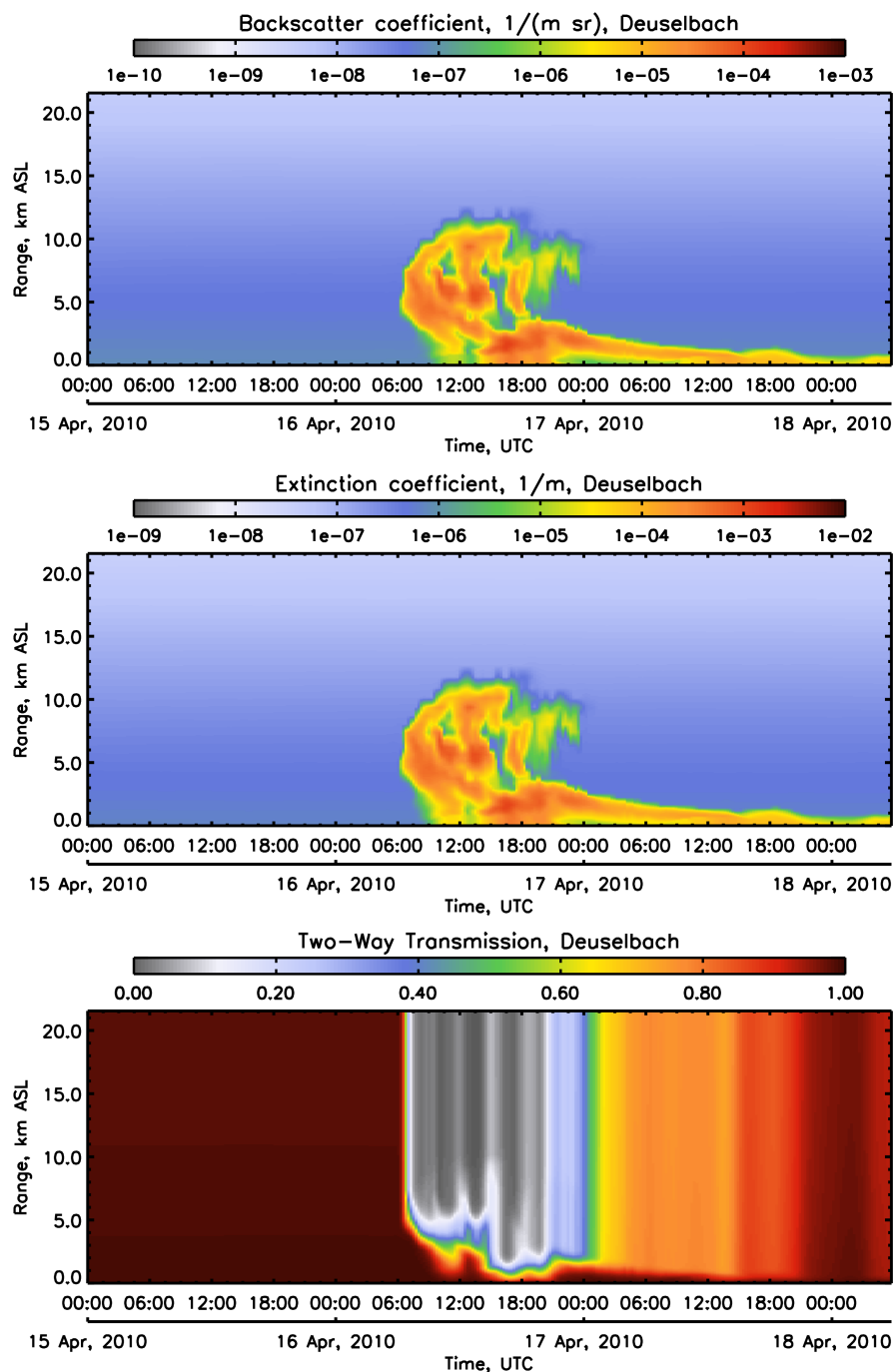
Figure 14. Time-height cross section of total extinction coefficient, backscatter coefficient, and two-way transmission, calculated by the forward model based on COSMO-ART output at the station Deuselbach (West Germany). The forward model represents clean air molecules and volcanic ash particles (no clouds, rain, fog, background aerosol or other scattering objects).
