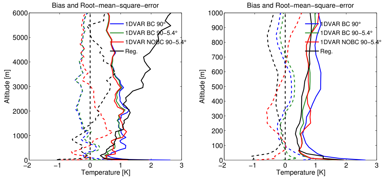
Figure 9. Vertical profiles of bias (dashed lines) and root-mean-square-errors (solid lines) of MWR retrievals against radiosondes: 1DVAR retrievals from AROME 1h forecasts, all elevation angles and bias correction (green), all elevation angles but no bias correction (red), only zenith angle and bias correction (blue) and linear regressions (black). Results on 56 clear-sky temperature profiles.
