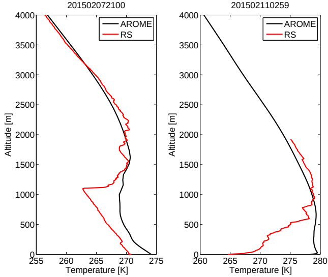
Figure 4. Temperature profiles observed by the radiosonde (red line) or extracted from the AROME analyses (black line): during unstable conditions the 07th of February at 21 UTC (left panel) and during the most stable period the 11th of February at 03 UTC (right panel). Altitudes are given in m above ground level.
