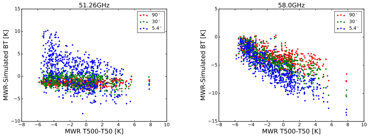
Figure 6. Observation minus background (AROME forecasts) departures as a function of HATPRO temperature differences between 500 m and 50 m and different elevation angles from 90 ° to 5.4 °.
