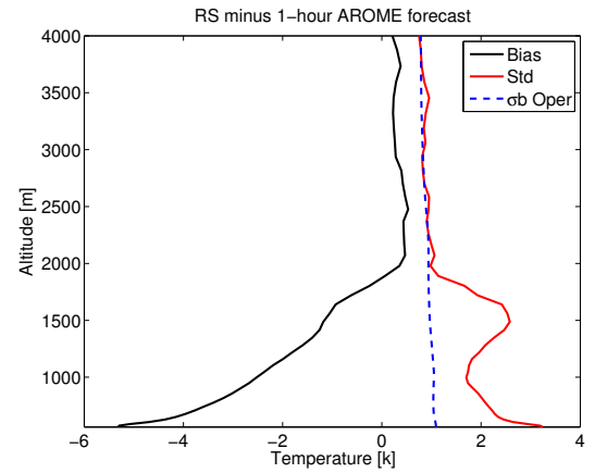
Figure 8. Bias (black line), standard deviation (red line) of the radiosonde minus 1h-AROME temperature differences. The operational background error used in AROME for the assimilation of satellite data is shown as the blue dashed line.
