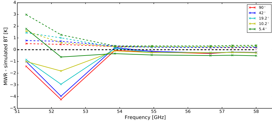
Figure 7. Observation minus background departures from radiosondes combined with AROME analyses for different elevation angles from 90^\circ to 5.4^\circ (coloured lines). For each angle, the bias is shown in solid line and the standard deviation in dashed line.
